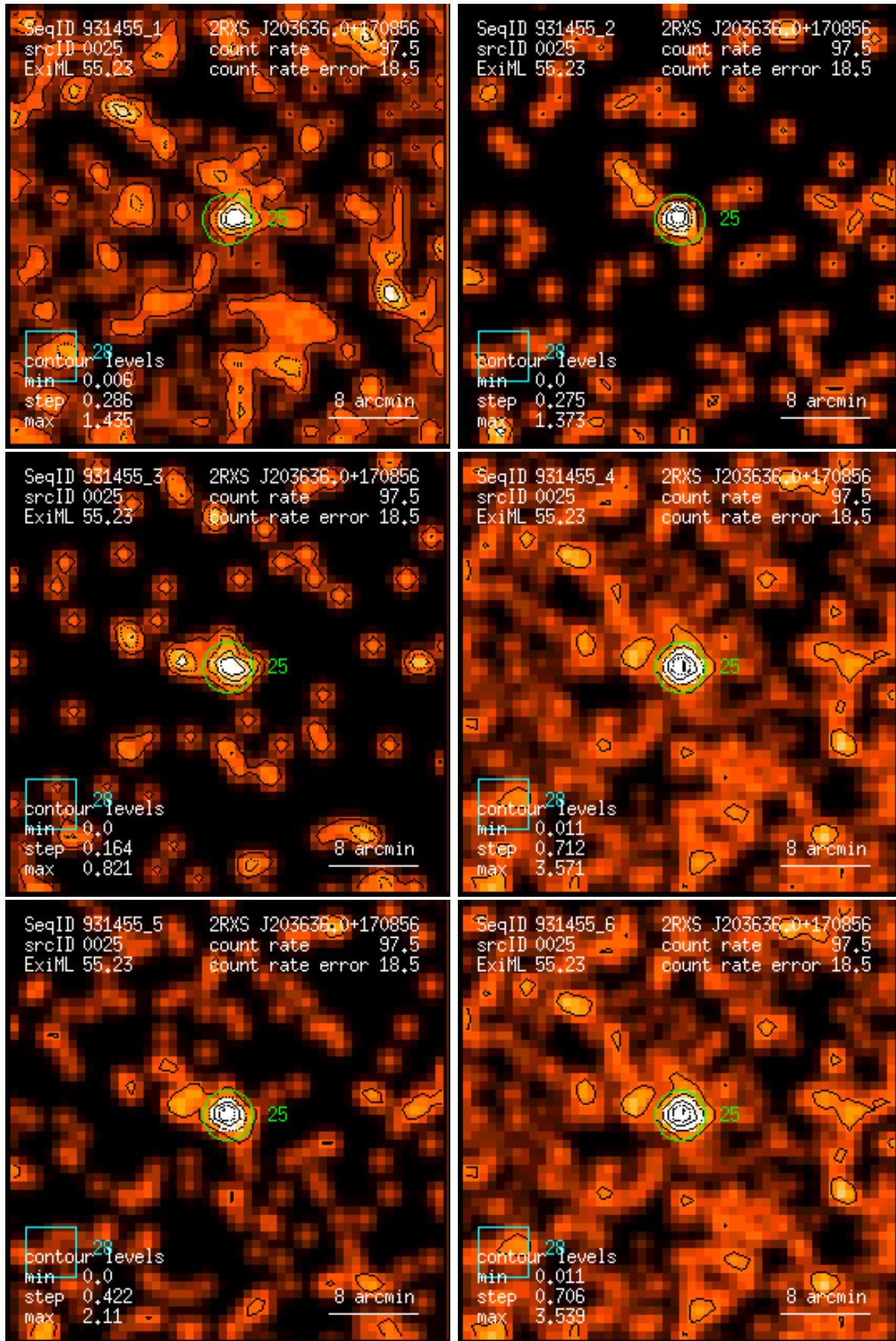
Figure 25: RASS 931455: detection 0025: band rate images, Gaussian filter: (1) PSPC channels 11 – 41, (2) 52 – 90, (3) 91 – 201, (4) 11 – 235, (5) 52 – 201, (6) 11 – 201. Broad band rates in counts/ks. Band rate contour levels in counts/ks/arcmin 2 .
