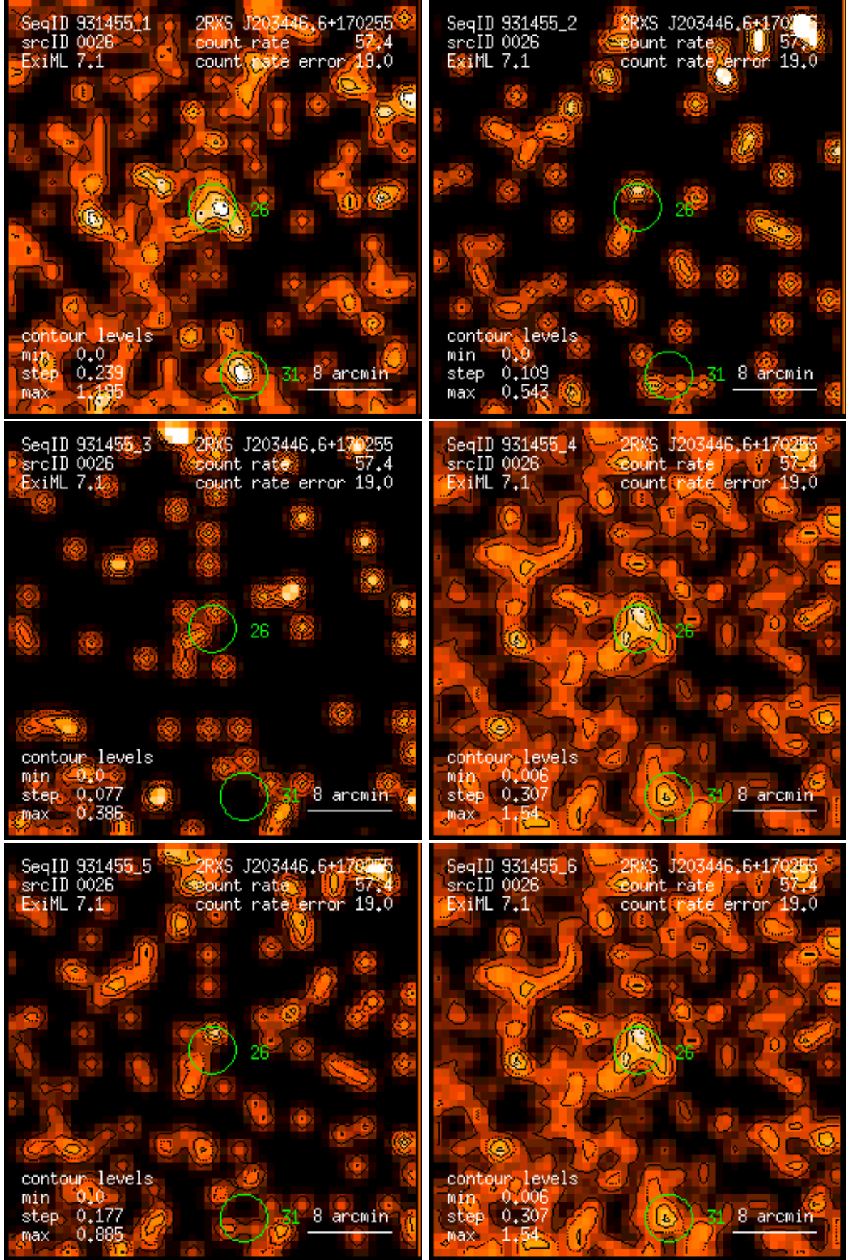
Figure 26: RASS 931455: detection 0026: band rate images, Gaussian filter: (1) PSPC channels 11 – 41, (2) 52 – 90, (3) 91 – 201, (4) 11 – 235, (5) 52 – 201, (6) 11 – 201. Broad band rates in counts/ks. Band rate contour levels in counts/ks/arcmin 2 .
