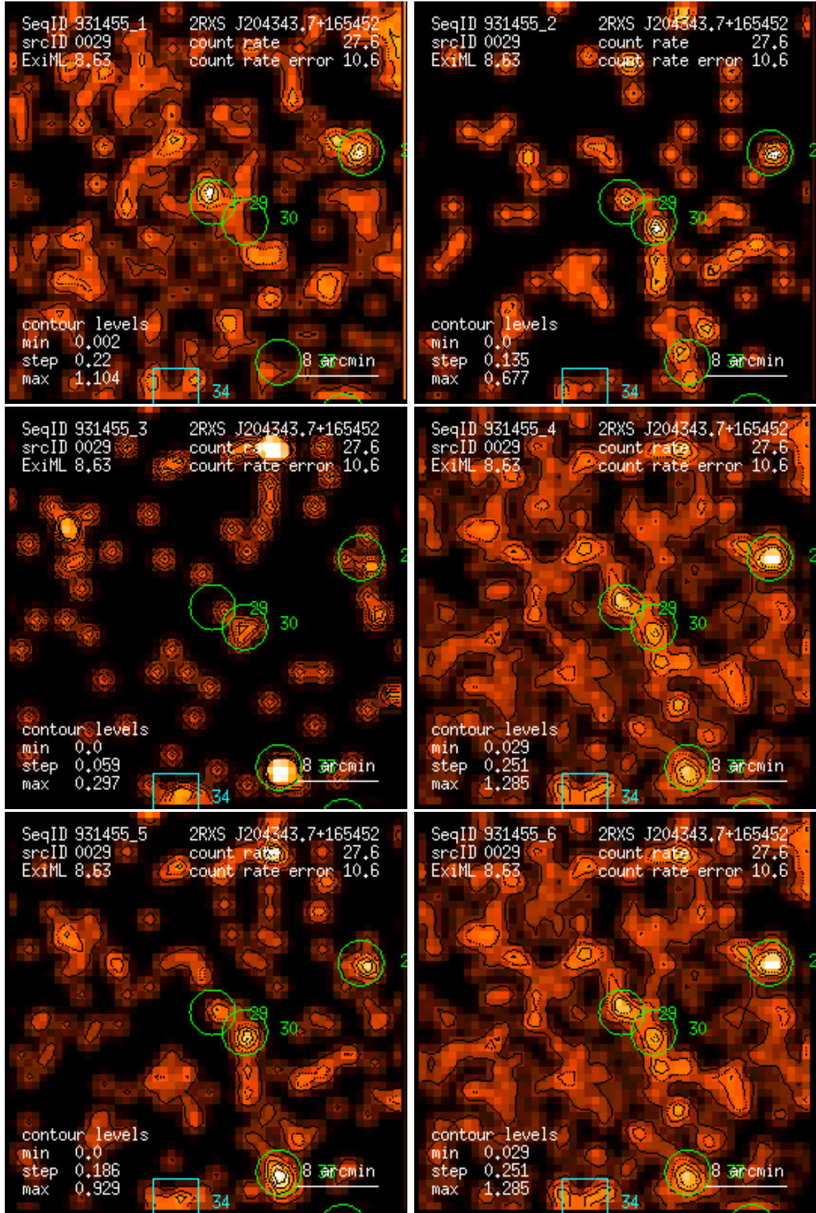
Figure 29: RASS 931455: detection 0029: band rate images, Gaussian filter: (1) PSPC channels 11 – 41, (2) 52 – 90, (3) 91 – 201, (4) 11 – 235, (5) 52 – 201, (6) 11 – 201. Broad band rates in counts/ks. Band rate contour levels in counts/ks/arcmin 2 .
