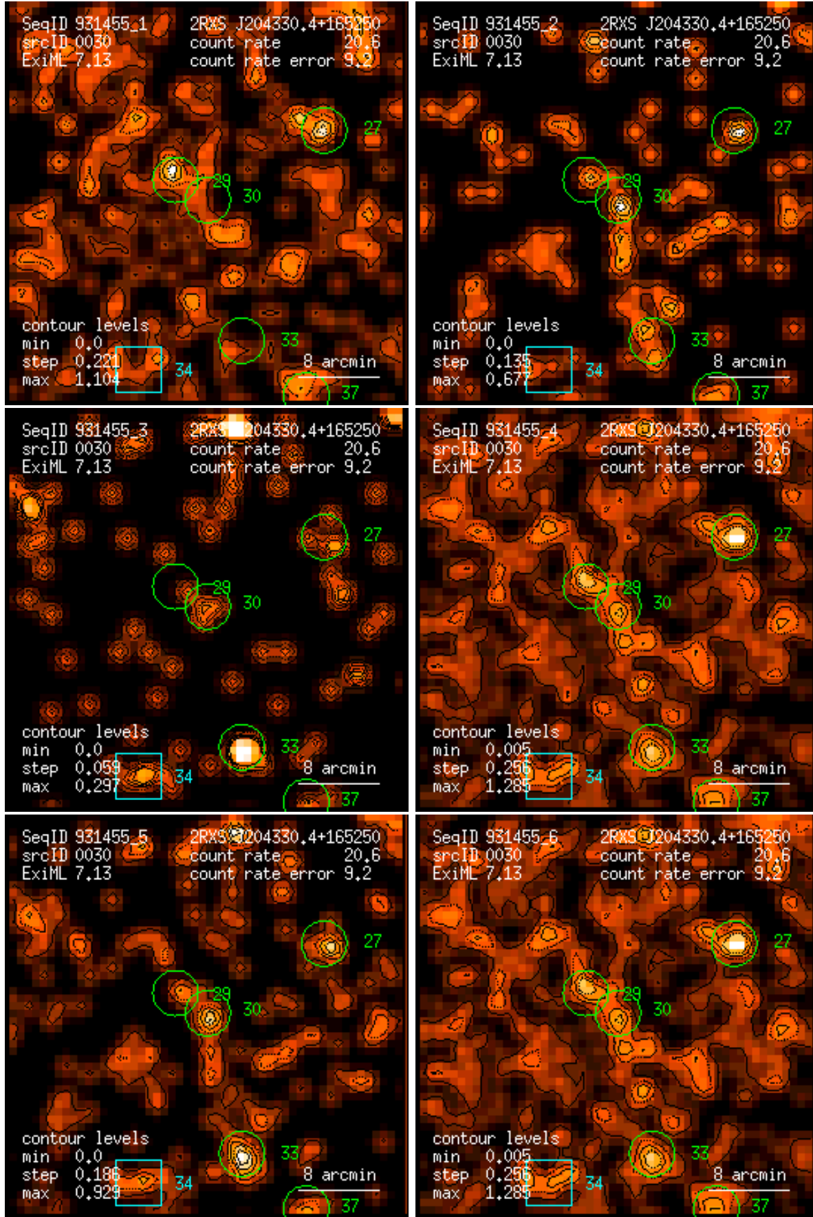
Figure 30: RASS 931455: detection 0030: band rate images, Gaussian filter: (1) PSPC channels 11 – 41, (2) 52 – 90, (3) 91 – 201, (4) 11 – 235, (5) 52 – 201, (6) 11 – 201. Broad band rates in counts/ks. Band rate contour levels in counts/ks/arcmin 2 .
