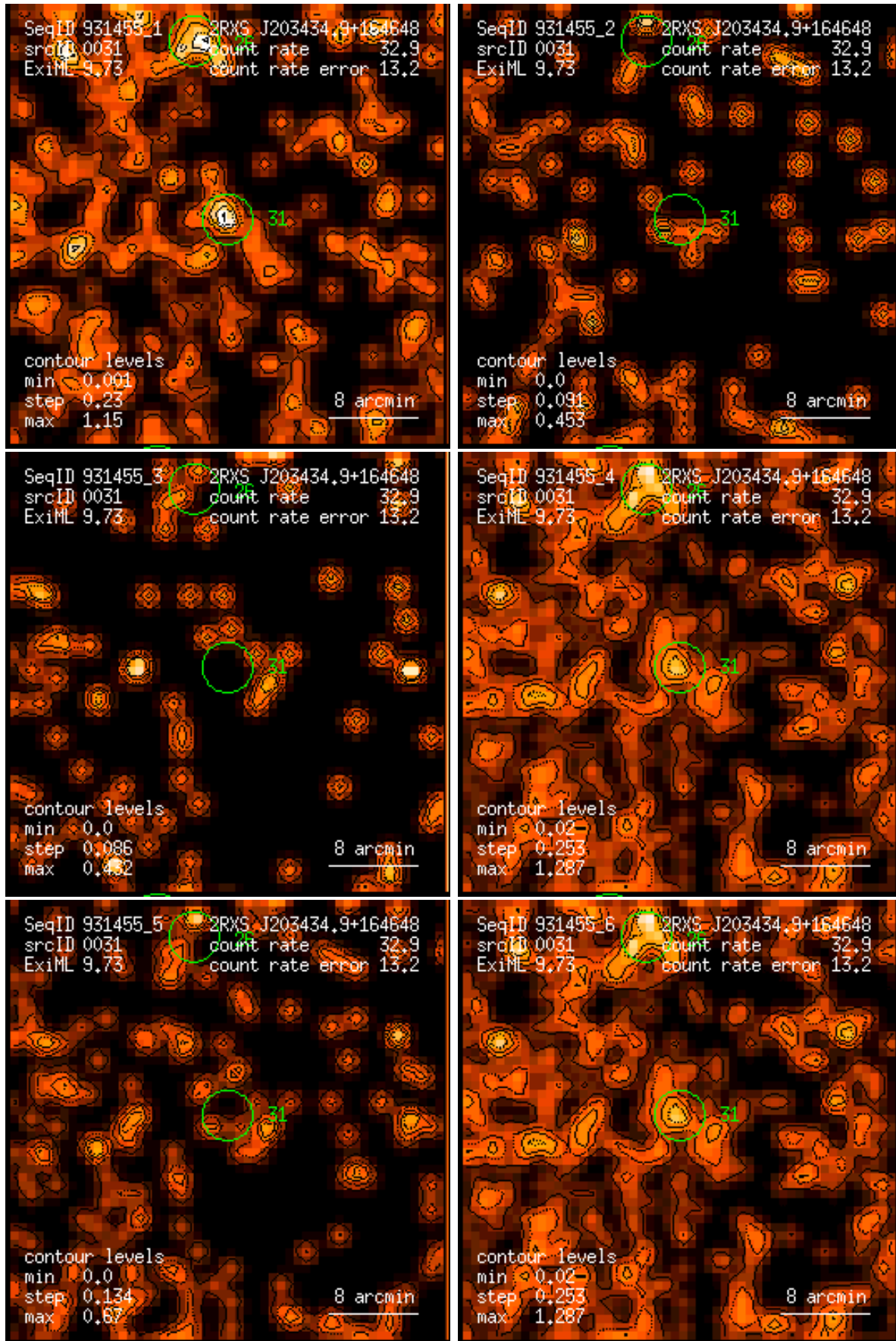
Figure 31: RASS 931455: detection 0031: band rate images, Gaussian filter: (1) PSPC channels 11 – 41, (2) 52 – 90, (3) 91 – 201, (4) 11 – 235, (5) 52 – 201, (6) 11 – 201. Broad band rates in counts/ks. Band rate contour levels in counts/ks/arcmin 2 .
