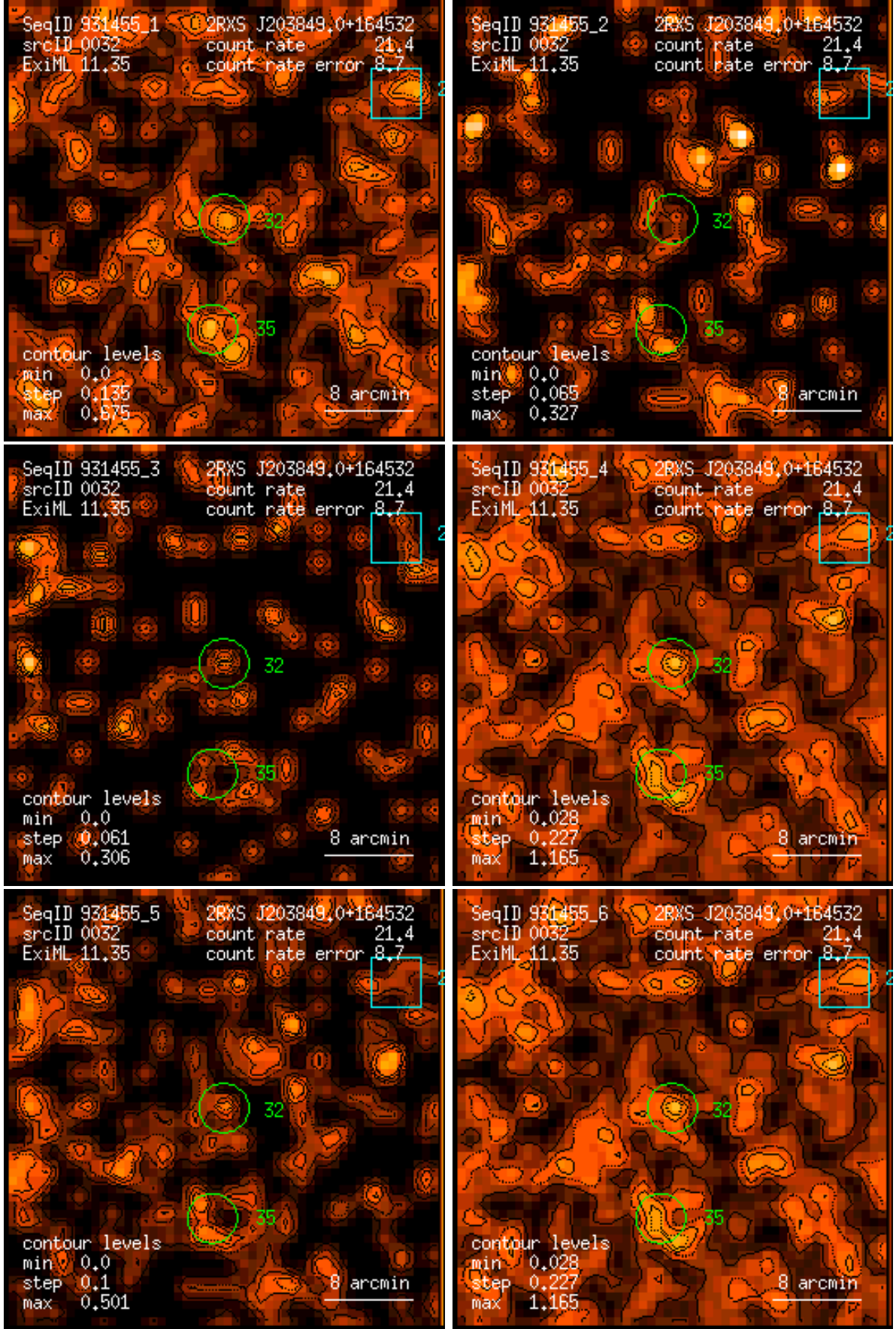
Figure 32: RASS 931455: detection 0032: band rate images, Gaussian filter: (1) PSPC channels 11 – 41, (2) 52 – 90, (3) 91 – 201, (4) 11 – 235, (5) 52 – 201, (6) 11 – 201. Broad band rates in counts/ks. Band rate contour levels in counts/ks/arcmin 2 .
