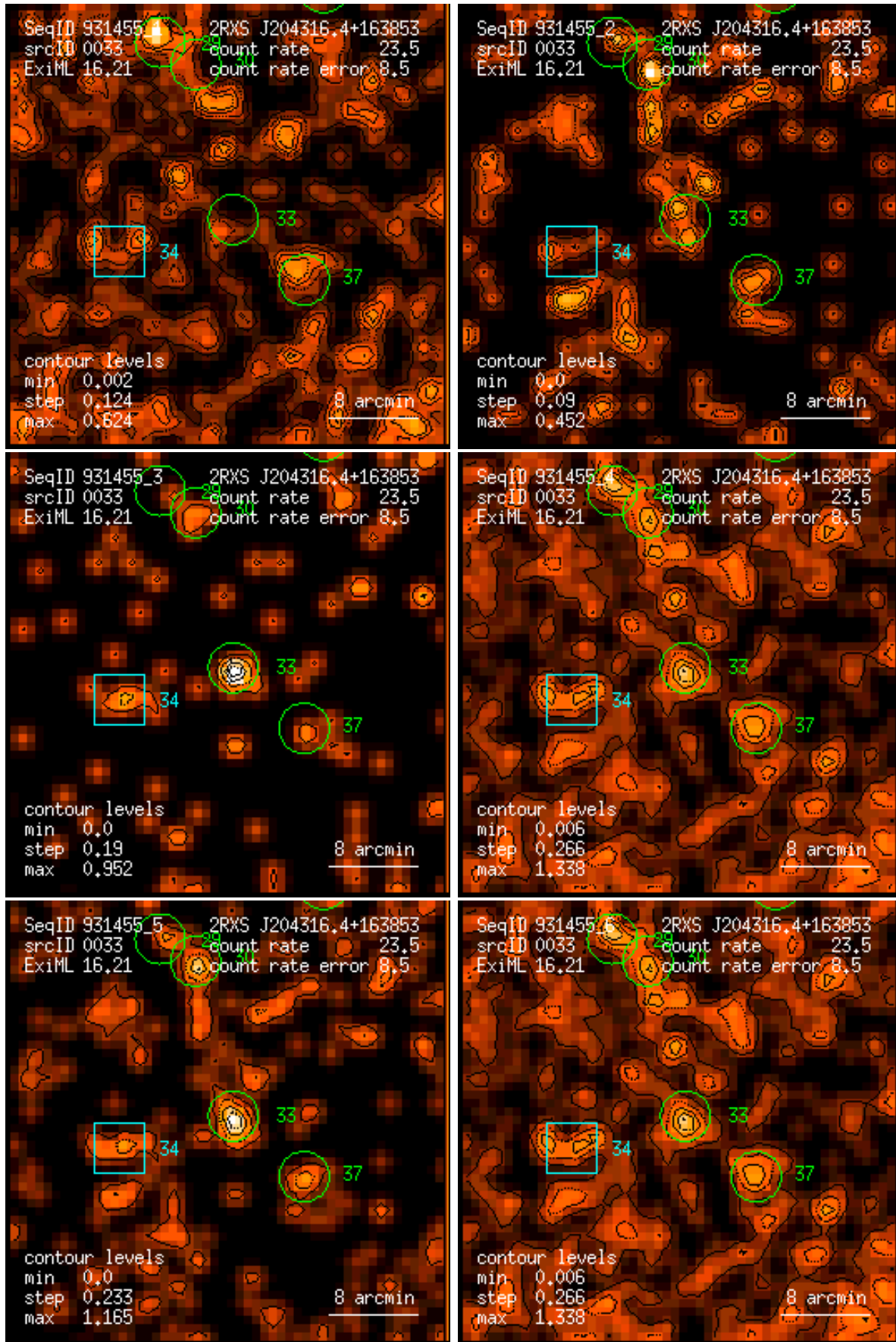
Figure 33: RASS 931455: detection 0033: band rate images, Gaussian filter: (1) PSPC channels 11 – 41, (2) 52 – 90, (3) 91 – 201, (4) 11 – 235, (5) 52 – 201, (6) 11 – 201. Broad band rates in counts/ks. Band rate contour levels in counts/ks/arcmin 2 .
