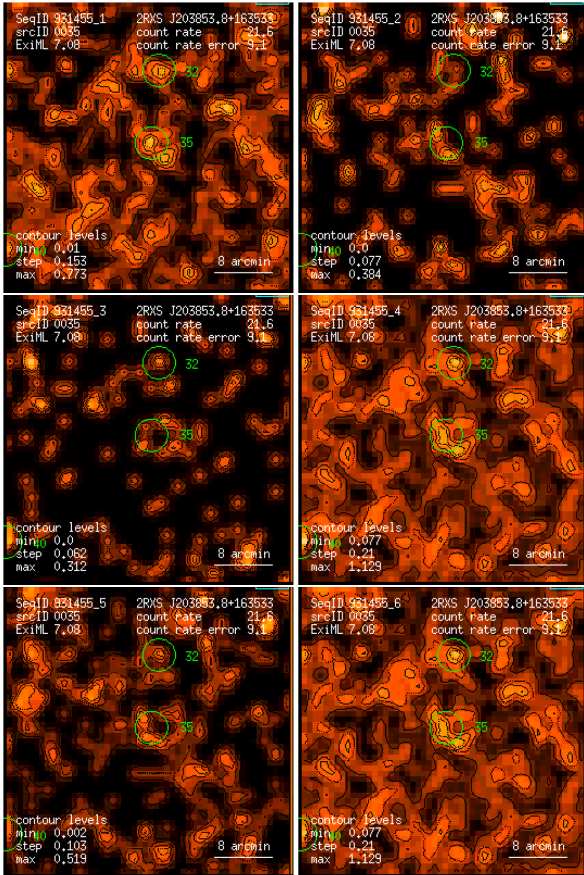
Figure 35: RASS 931455: detection 0035: band rate images, Gaussian filter: (1) PSPC channels 11 – 41, (2) 52 – 90, (3) 91 – 201, (4) 11 – 235, (5) 52 – 201, (6) 11 – 201. Broad band rates in counts/ks. Band rate contour levels in counts/ks/arcmin 2 .
