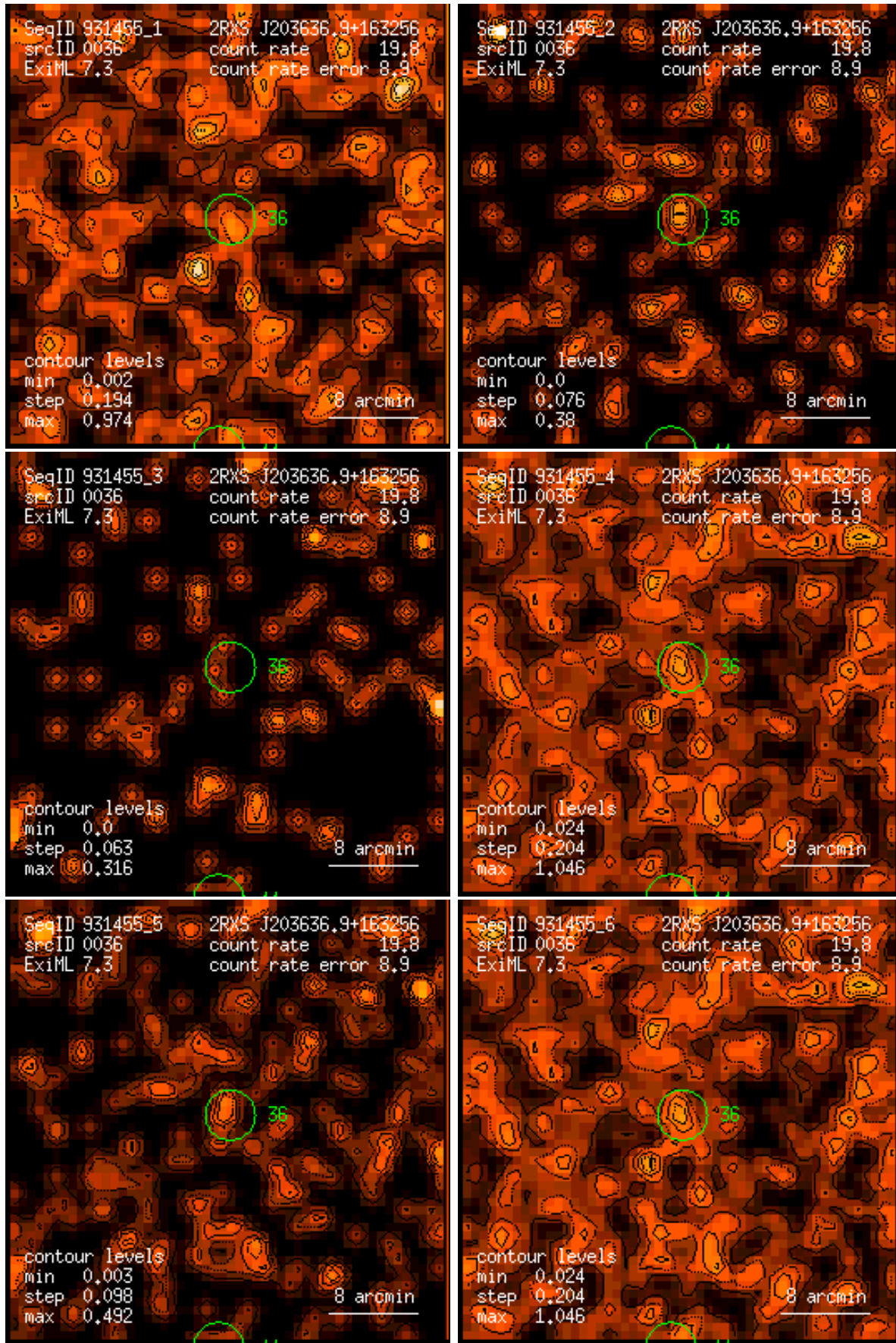
Figure 36: RASS 931455: detection 0036: band rate images, Gaussian filter: (1) PSPC channels 11 – 41, (2) 52 – 90, (3) 91 – 201, (4) 11 – 235, (5) 52 – 201, (6) 11 – 201. Broad band rates in counts/ks. Band rate contour levels in counts/ks/arcmin 2 .
