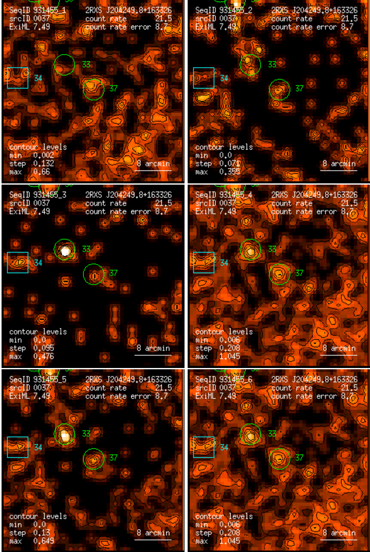
Figure 37: RASS 931455: detection 0037: band rate images, Gaussian filter: (1) PSPC channels 11 – 41, (2) 52 – 90, (3) 91 – 201, (4) 11 – 235, (5) 52 – 201, (6) 11 – 201. Broad band rates in counts/ks. Band rate contour levels in counts/ks/arcmin 2 .
