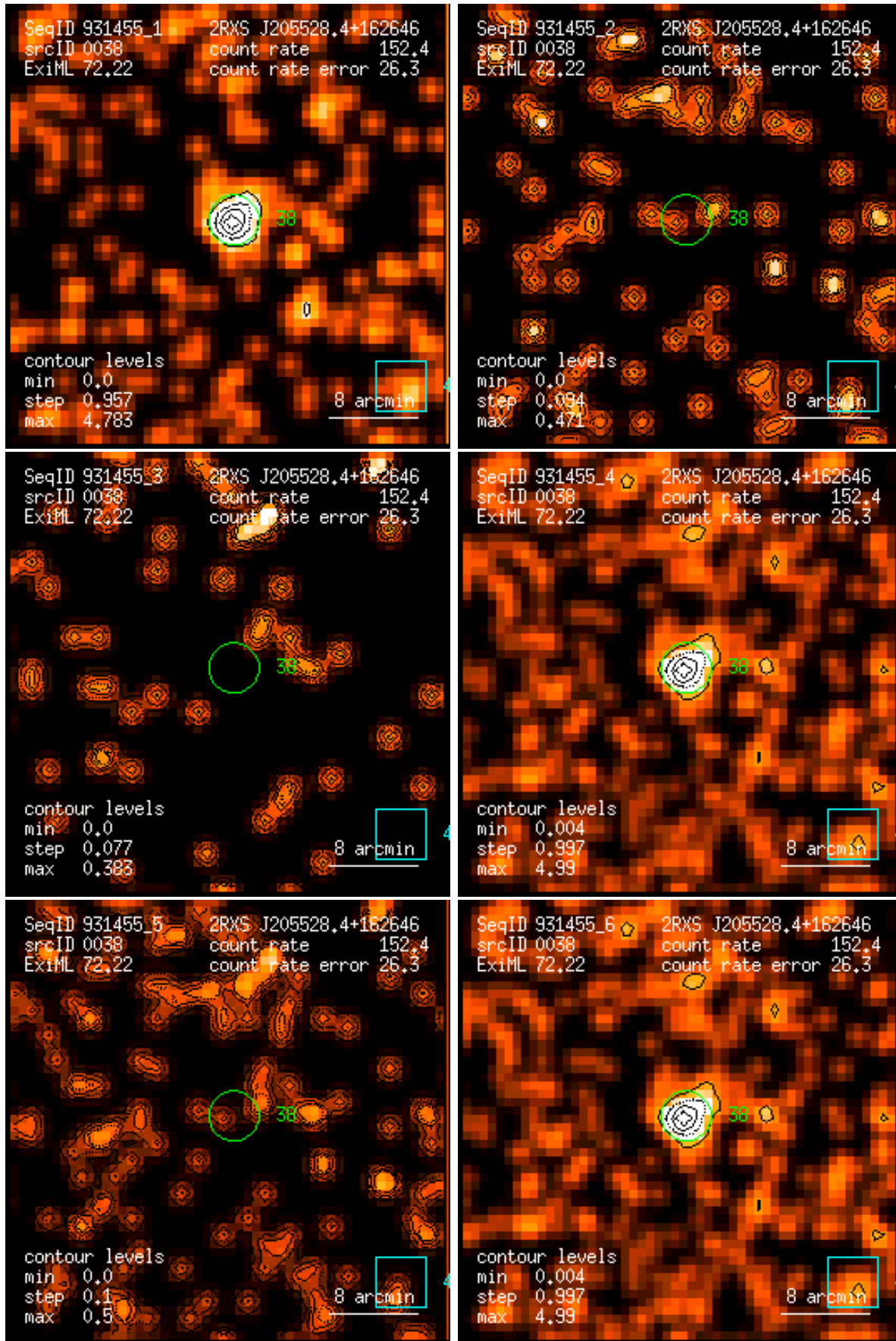
Figure 38: RASS 931455: detection 0038: band rate images, Gaussian filter: (1) PSPC channels 11 – 41, (2) 52 – 90, (3) 91 – 201, (4) 11 – 235, (5) 52 – 201, (6) 11 – 201. Broad band rates in counts/ks. Band rate contour levels in counts/ks/arcmin 2 .
