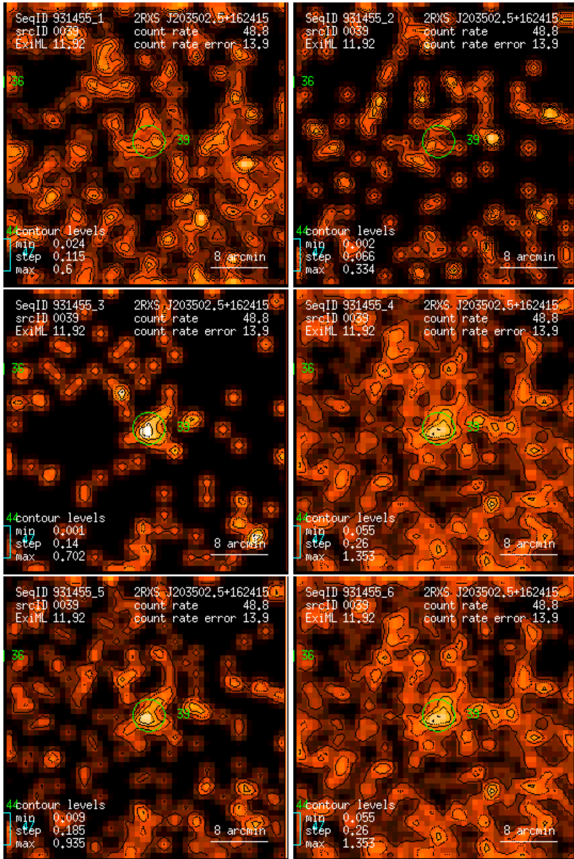
Figure 39: RASS 931455: detection 0039: band rate images, Gaussian filter: (1) PSPC channels 11 – 41, (2) 52 – 90, (3) 91 – 201, (4) 11 – 235, (5) 52 – 201, (6) 11 – 201. Broad band rates in counts/ks. Band rate contour levels in counts/ks/arcmin 2 .
