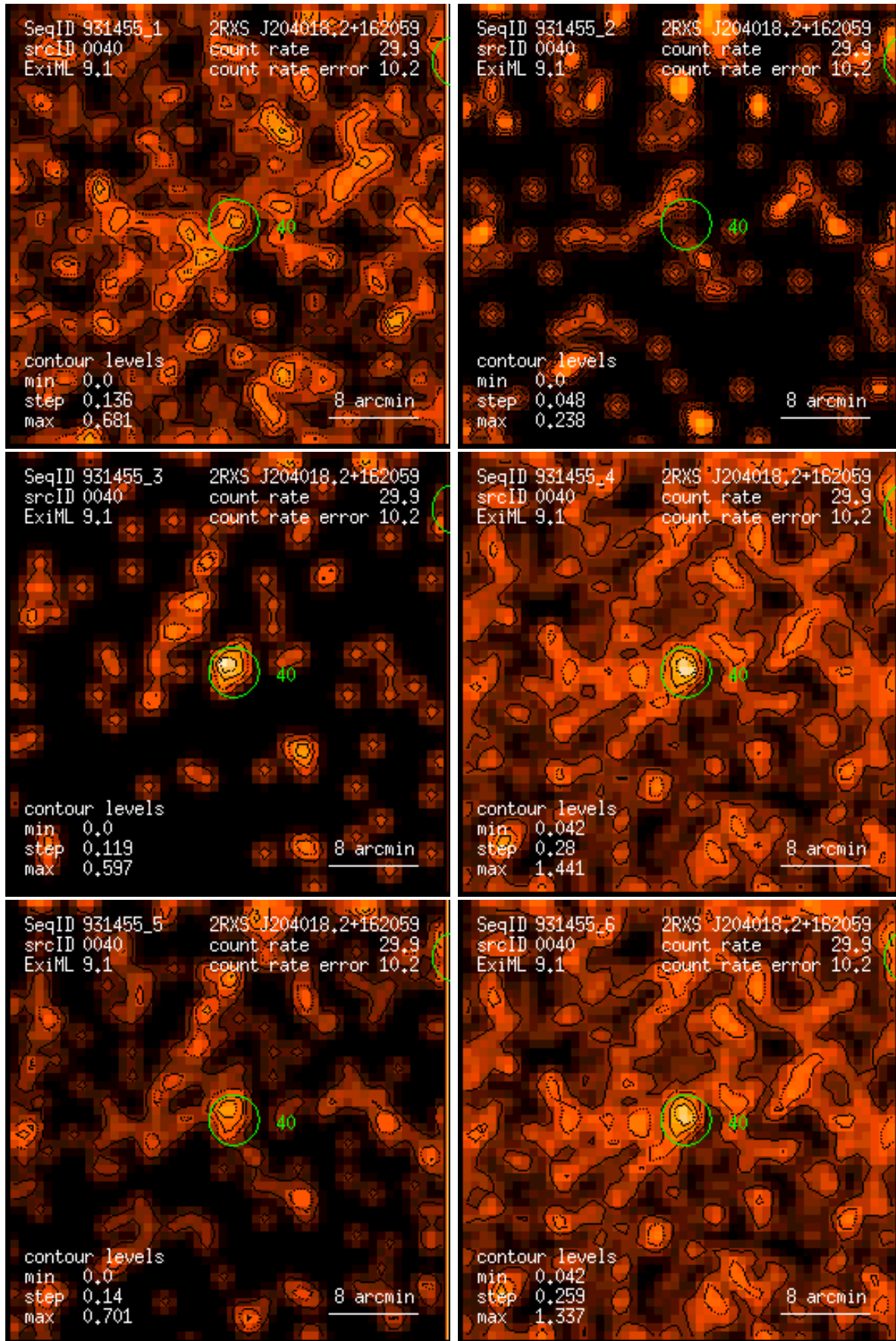
Figure 40: RASS 931455: detection 0040: band rate images, Gaussian filter: (1) PSPC channels 11 – 41, (2) 52 – 90, (3) 91 – 201, (4) 11 – 235, (5) 52 – 201, (6) 11 – 201. Broad band rates in counts/ks. Band rate contour levels in counts/ks/arcmin 2 .
