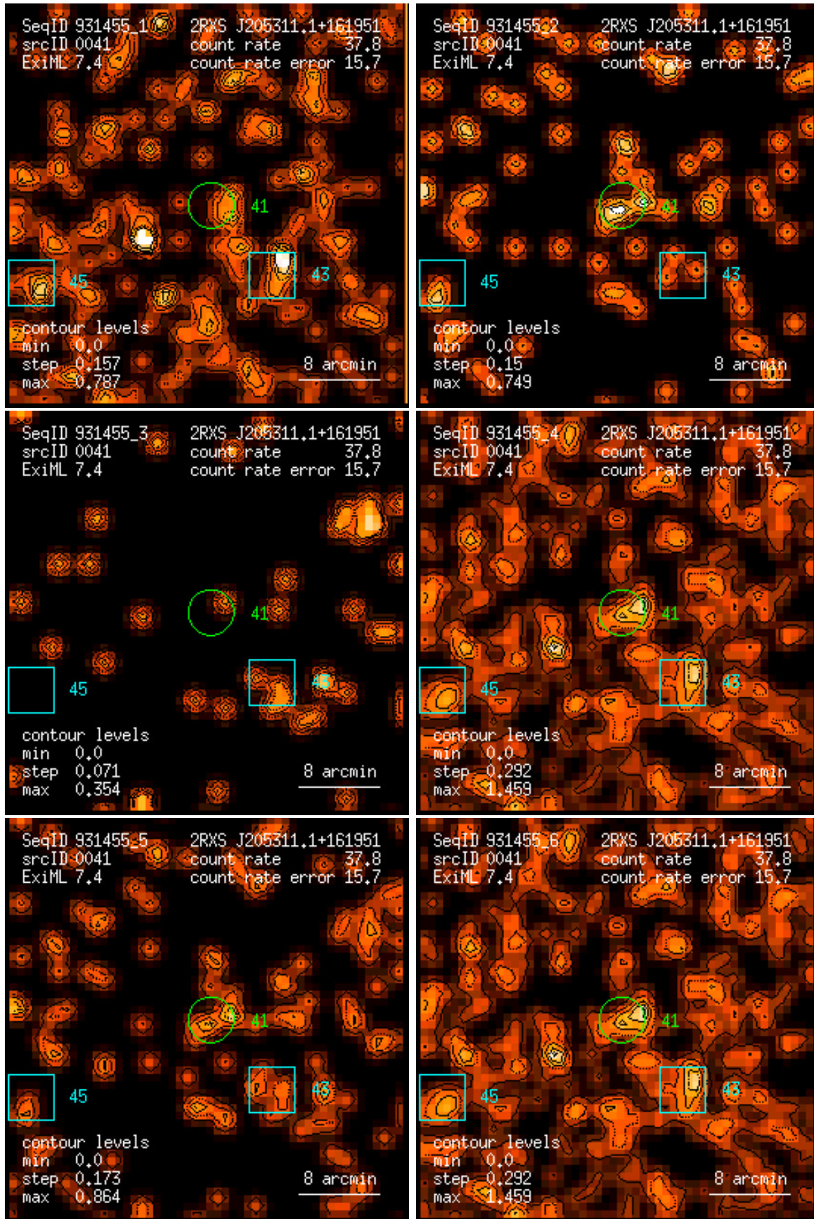
Figure 41: RASS 931455: detection 0041: band rate images, Gaussian filter: (1) PSPC channels 11 – 41, (2) 52 – 90, (3) 91 – 201, (4) 11 – 235, (5) 52 – 201, (6) 11 – 201. Broad band rates in counts/ks. Band rate contour levels in counts/ks/arcmin 2 .
