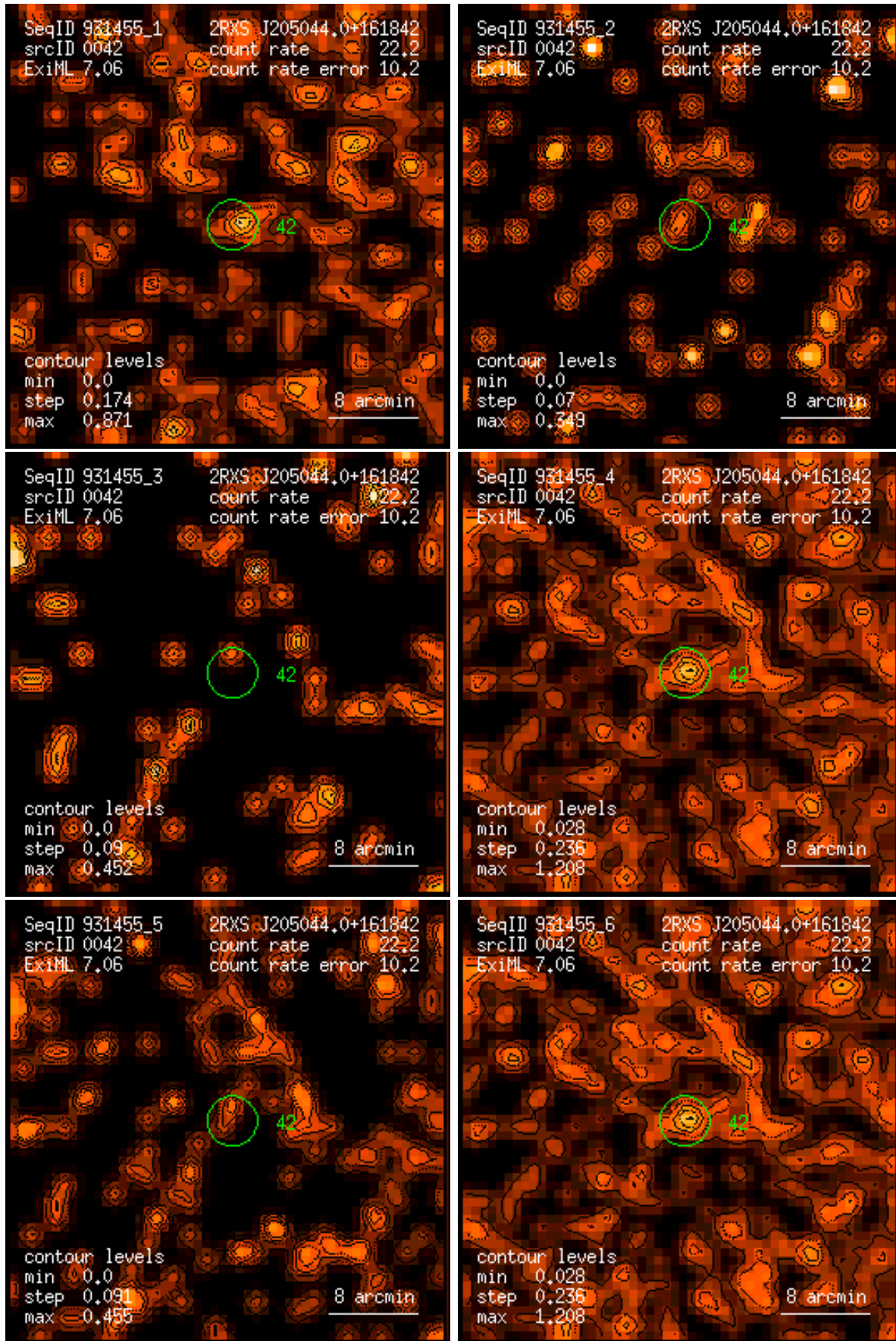
Figure 42: RASS 931455: detection 0042: band rate images, Gaussian filter: (1) PSPC channels 11 – 41, (2) 52 – 90, (3) 91 – 201, (4) 11 – 235, (5) 52 – 201, (6) 11 – 201. Broad band rates in counts/ks. Band rate contour levels in counts/ks/arcmin 2 .
