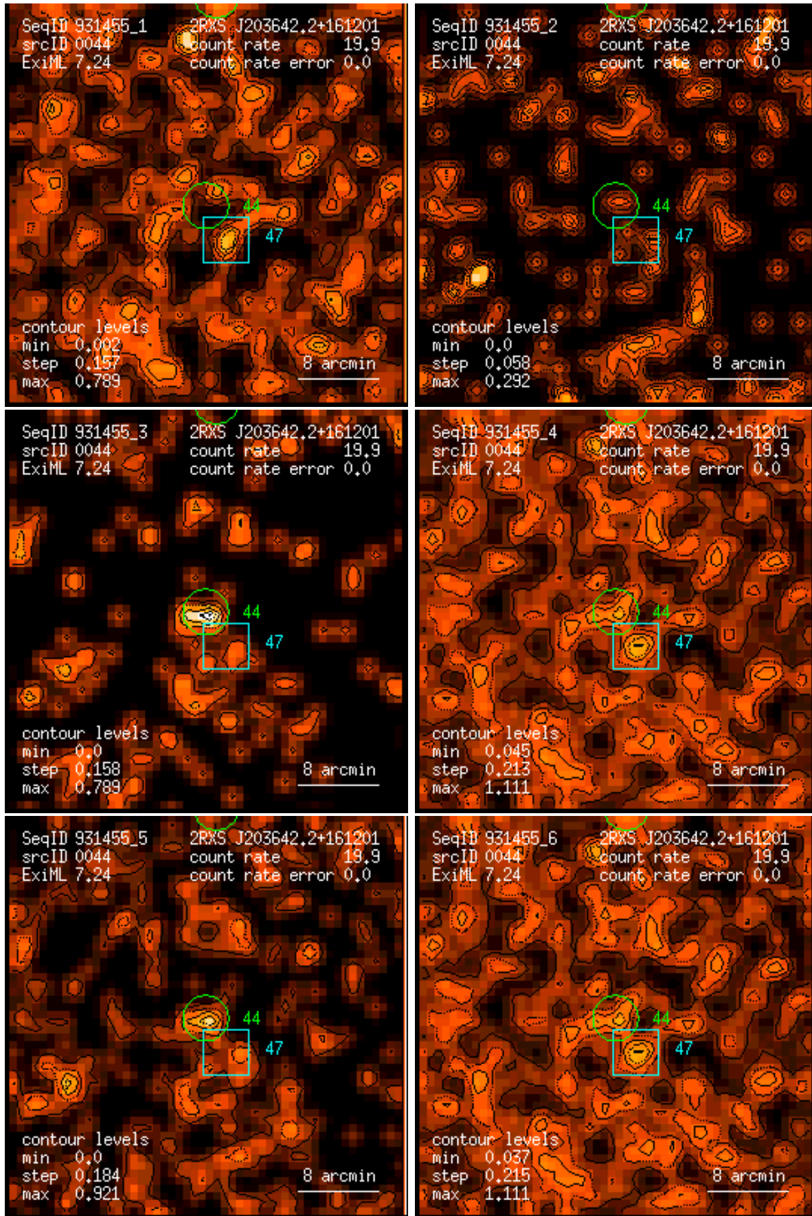
Figure 44: RASS 931455: detection 0044: band rate images, Gaussian filter: (1) PSPC channels 11 – 41, (2) 52 – 90, (3) 91 – 201, (4) 11 – 235, (5) 52 – 201, (6) 11 – 201. Broad band rates in counts/ks. Band rate contour levels in counts/ks/arcmin 2 .
