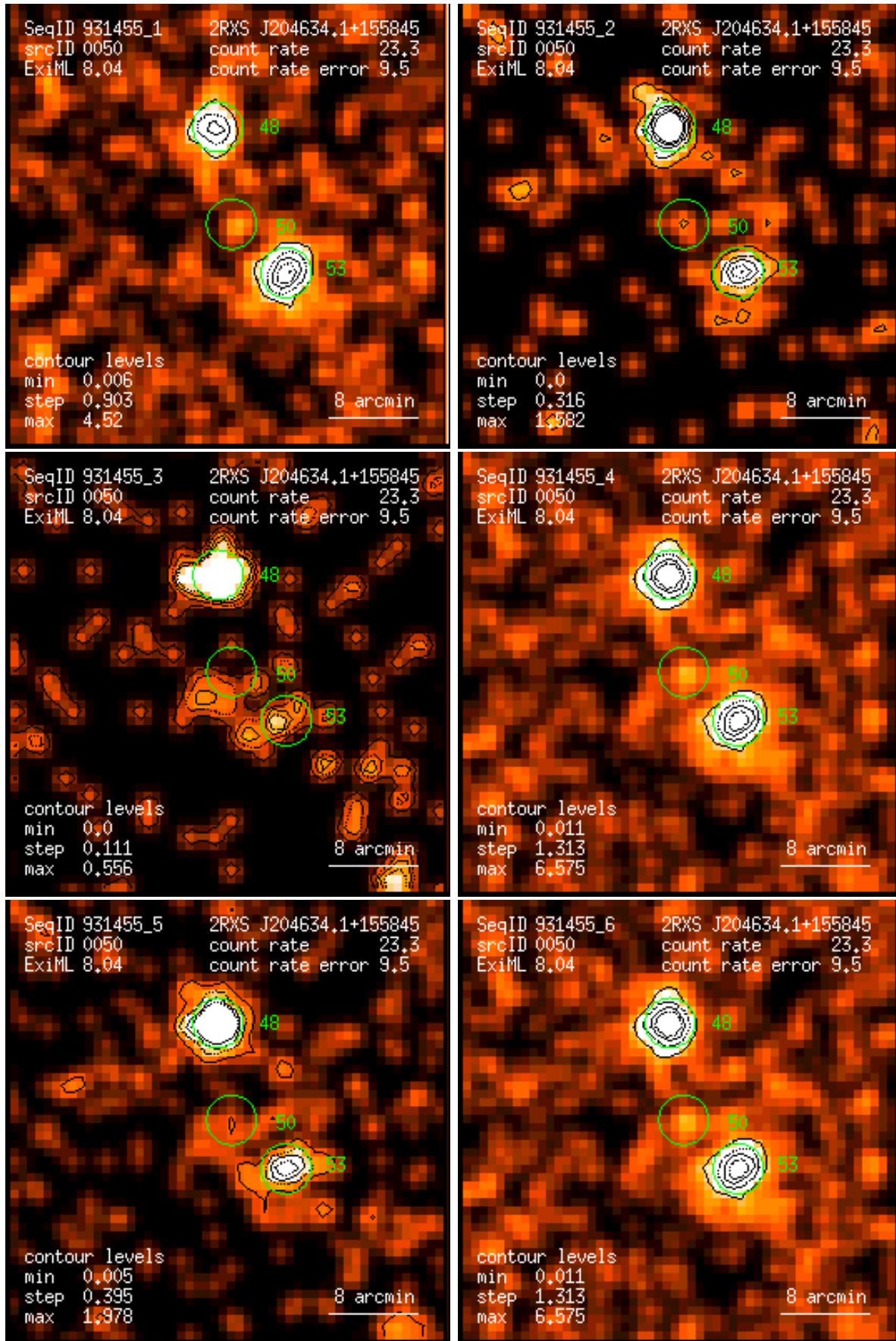
Figure 50: RASS 931455: detection 0050: band rate images, Gaussian filter: (1) PSPC channels 11 – 41, (2) 52 – 90, (3) 91 – 201, (4) 11 – 235, (5) 52 – 201, (6) 11 – 201. Broad band rates in counts/ks. Band rate contour levels in counts/ks/arcmin 2 .
