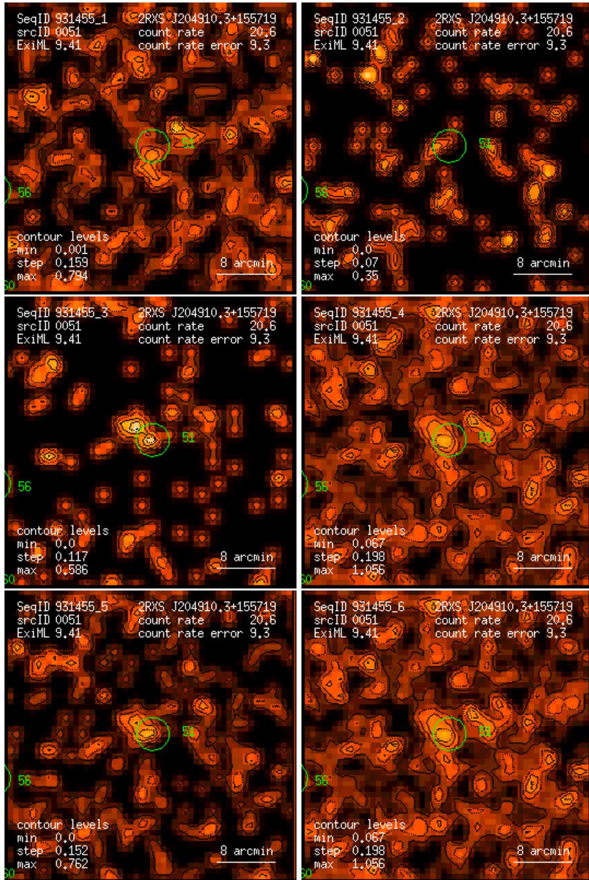
Figure 51: RASS 931455: detection 0051: band rate images, Gaussian filter: (1) PSPC channels 11 – 41, (2) 52 – 90, (3) 91 – 201, (4) 11 – 235, (5) 52 – 201, (6) 11 – 201. Broad band rates in counts/ks. Band rate contour levels in counts/ks/arcmin 2 .
