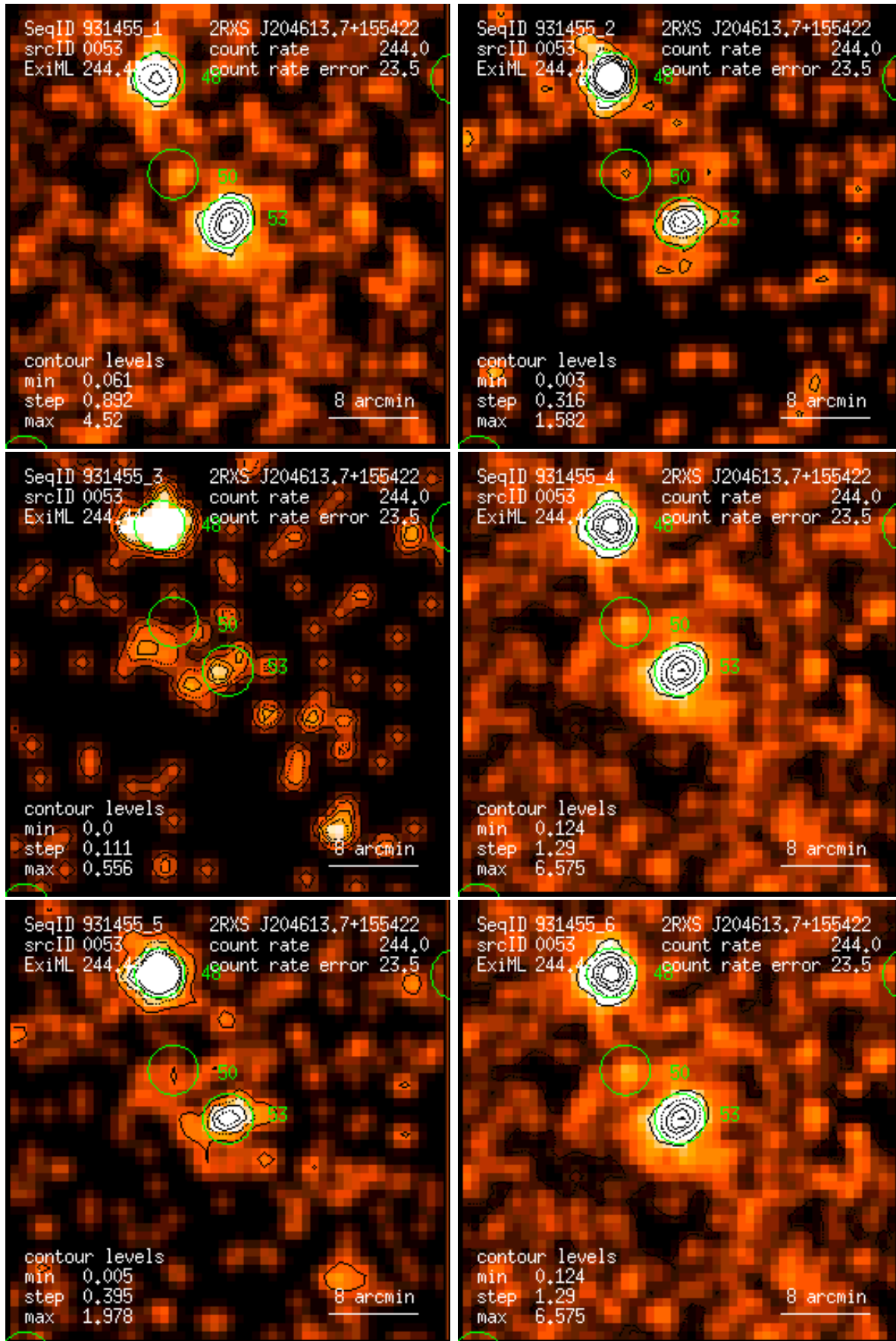
Figure 53: RASS 931455: detection 0053: band rate images, Gaussian filter: (1) PSPC channels 11 – 41, (2) 52 – 90, (3) 91 – 201, (4) 11 – 235, (5) 52 – 201, (6) 11 – 201. Broad band rates in counts/ks. Band rate contour levels in counts/ks/arcmin 2 .
