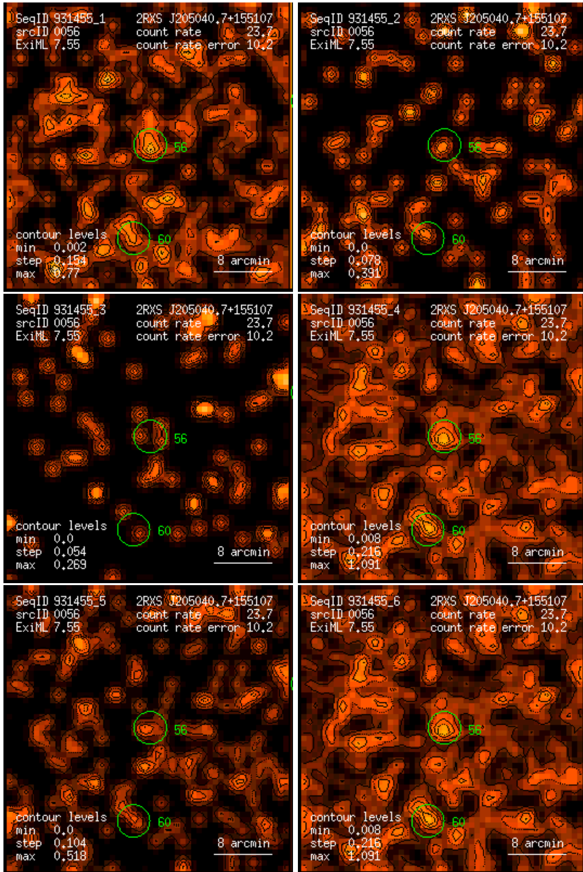
Figure 56: RASS 931455: detection 0056: band rate images, Gaussian filter: (1) PSPC channels 11 – 41, (2) 52 – 90, (3) 91 – 201, (4) 11 – 235, (5) 52 – 201, (6) 11 – 201. Broad band rates in counts/ks. Band rate contour levels in counts/ks/arcmin 2 .
