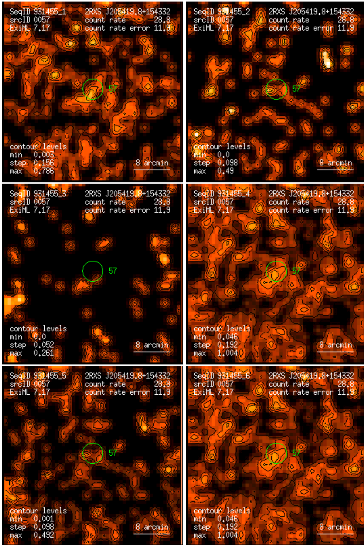
Figure 57: RASS 931455: detection 0057: band rate images, Gaussian filter: (1) PSPC channels 11 – 41, (2) 52 – 90, (3) 91 – 201, (4) 11 – 235, (5) 52 – 201, (6) 11 – 201. Broad band rates in counts/ks. Band rate contour levels in counts/ks/arcmin 2 .
