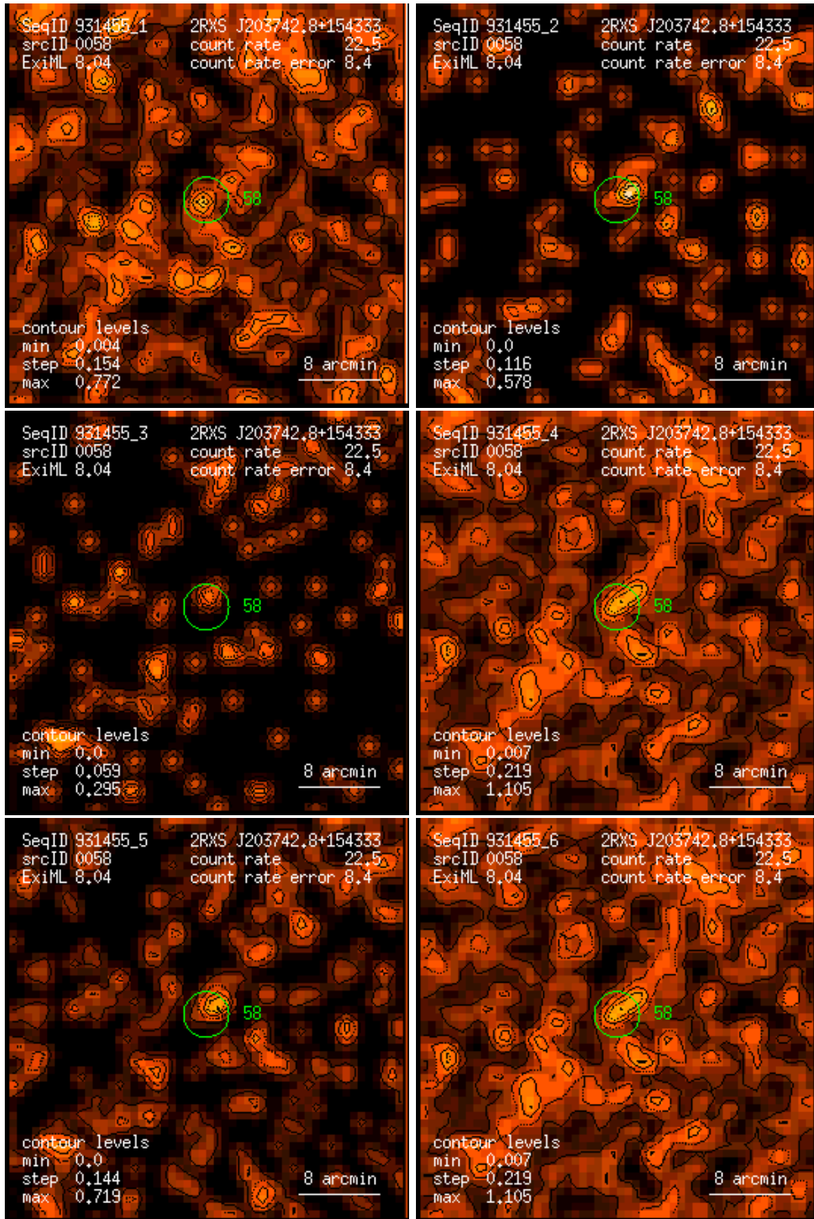
Figure 58: RASS 931455: detection 0058: band rate images, Gaussian filter: (1) PSPC channels 11 – 41, (2) 52 – 90, (3) 91 – 201, (4) 11 – 235, (5) 52 – 201, (6) 11 – 201. Broad band rates in counts/ks. Band rate contour levels in counts/ks/arcmin 2 .
