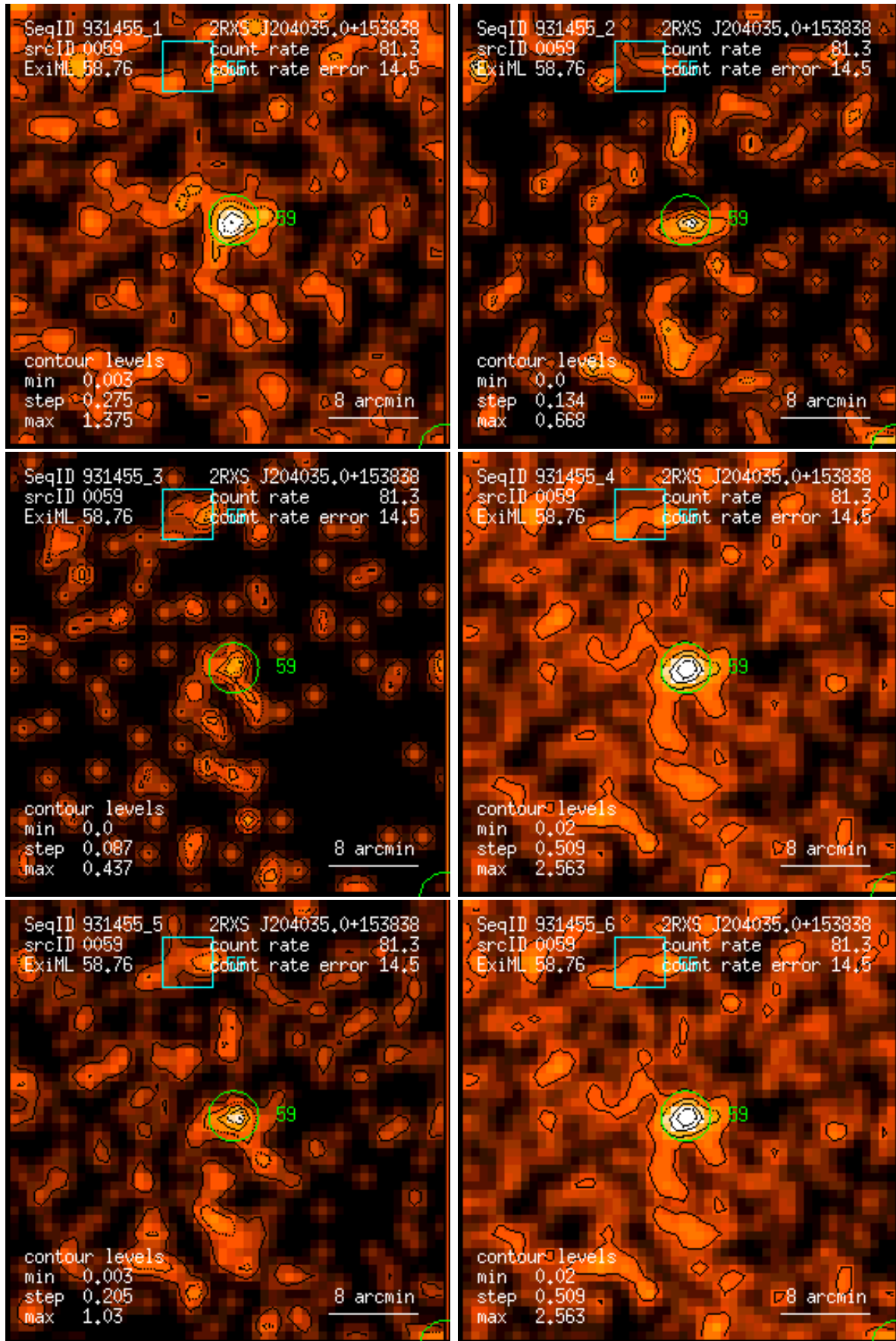
Figure 59: RASS 931455: detection 0059: band rate images, Gaussian filter: (1) PSPC channels 11 – 41, (2) 52 – 90, (3) 91 – 201, (4) 11 – 235, (5) 52 – 201, (6) 11 – 201. Broad band rates in counts/ks. Band rate contour levels in counts/ks/arcmin 2 .
