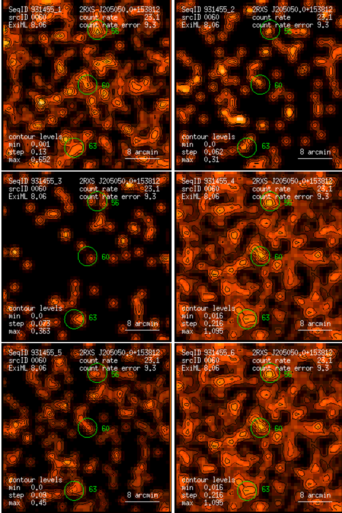
Figure 60: RASS 931455: detection 0060: band rate images, Gaussian filter: (1) PSPC channels 11 – 41, (2) 52 – 90, (3) 91 – 201, (4) 11 – 235, (5) 52 – 201, (6) 11 – 201. Broad band rates in counts/ks. Band rate contour levels in counts/ks/arcmin 2 .
