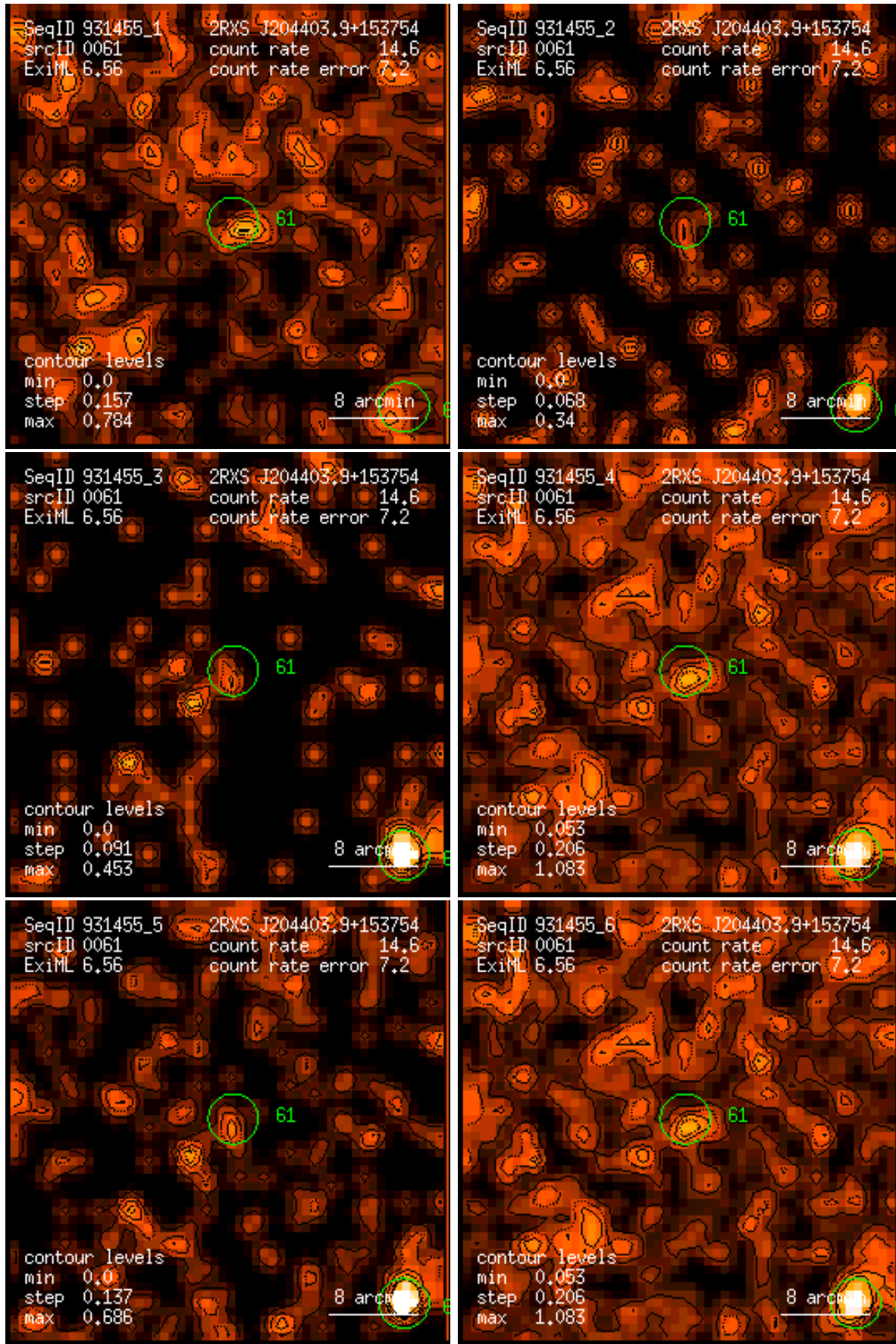
Figure 61: RASS 931455: detection 0061: band rate images, Gaussian filter: (1) PSPC channels 11 – 41, (2) 52 – 90, (3) 91 – 201, (4) 11 – 235, (5) 52 – 201, (6) 11 – 201. Broad band rates in counts/ks. Band rate contour levels in counts/ks/arcmin 2 .
