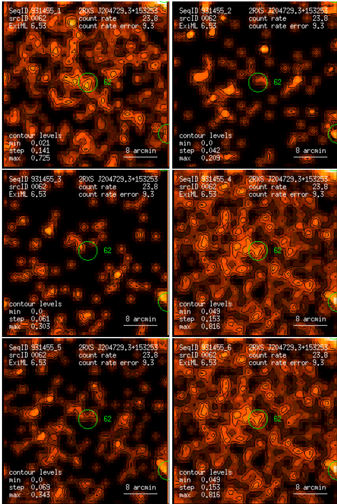
Figure 62: RASS 931455: detection 0062: band rate images, Gaussian filter: (1) PSPC channels 11 – 41, (2) 52 – 90, (3) 91 – 201, (4) 11 – 235, (5) 52 – 201, (6) 11 – 201. Broad band rates in counts/ks. Band rate contour levels in counts/ks/arcmin 2 .
