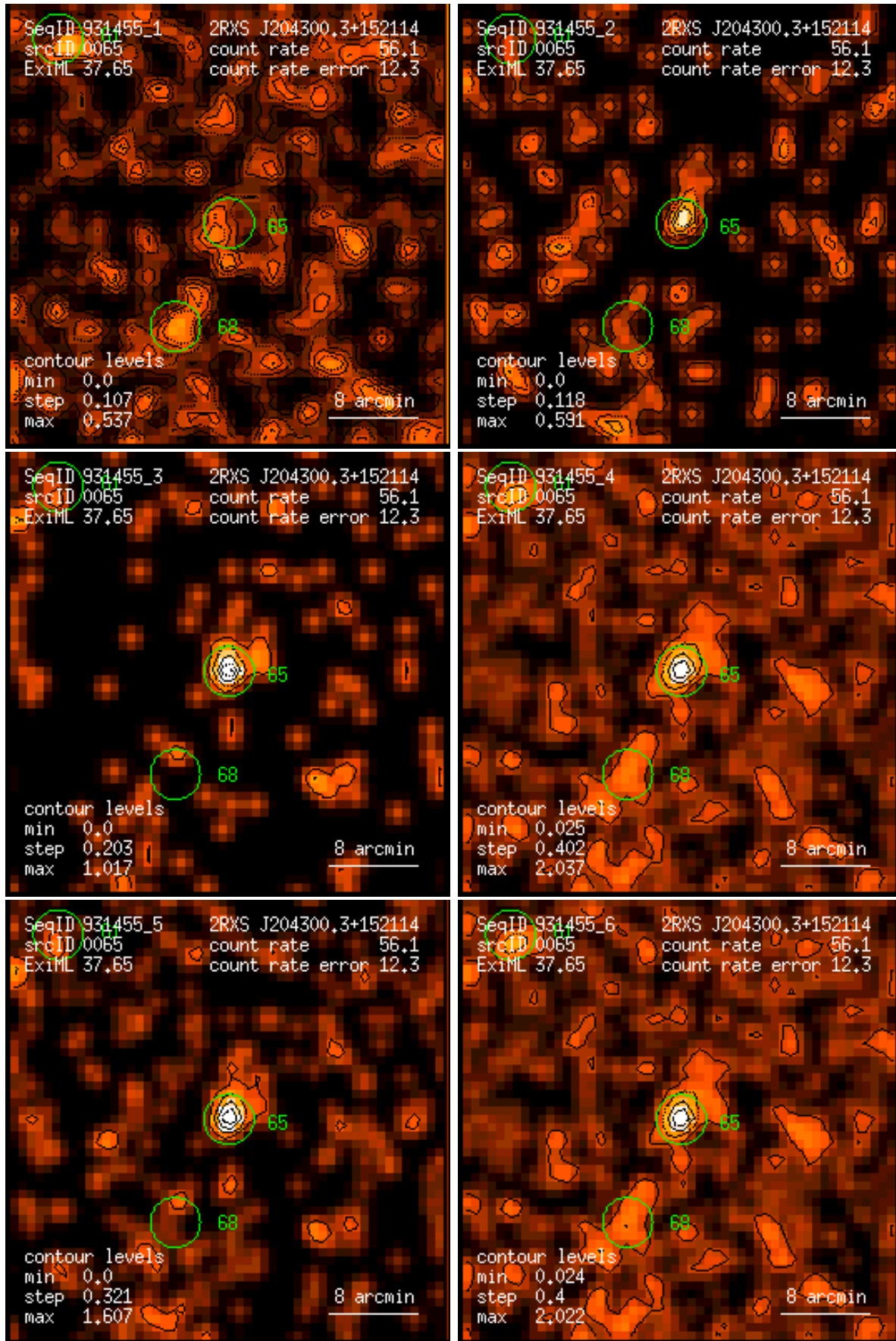
Figure 65: RASS 931455: detection 0065: band rate images, Gaussian filter: (1) PSPC channels 11 – 41, (2) 52 – 90, (3) 91 – 201, (4) 11 – 235, (5) 52 – 201, (6) 11 – 201. Broad band rates in counts/ks. Band rate contour levels in counts/ks/arcmin 2 .
