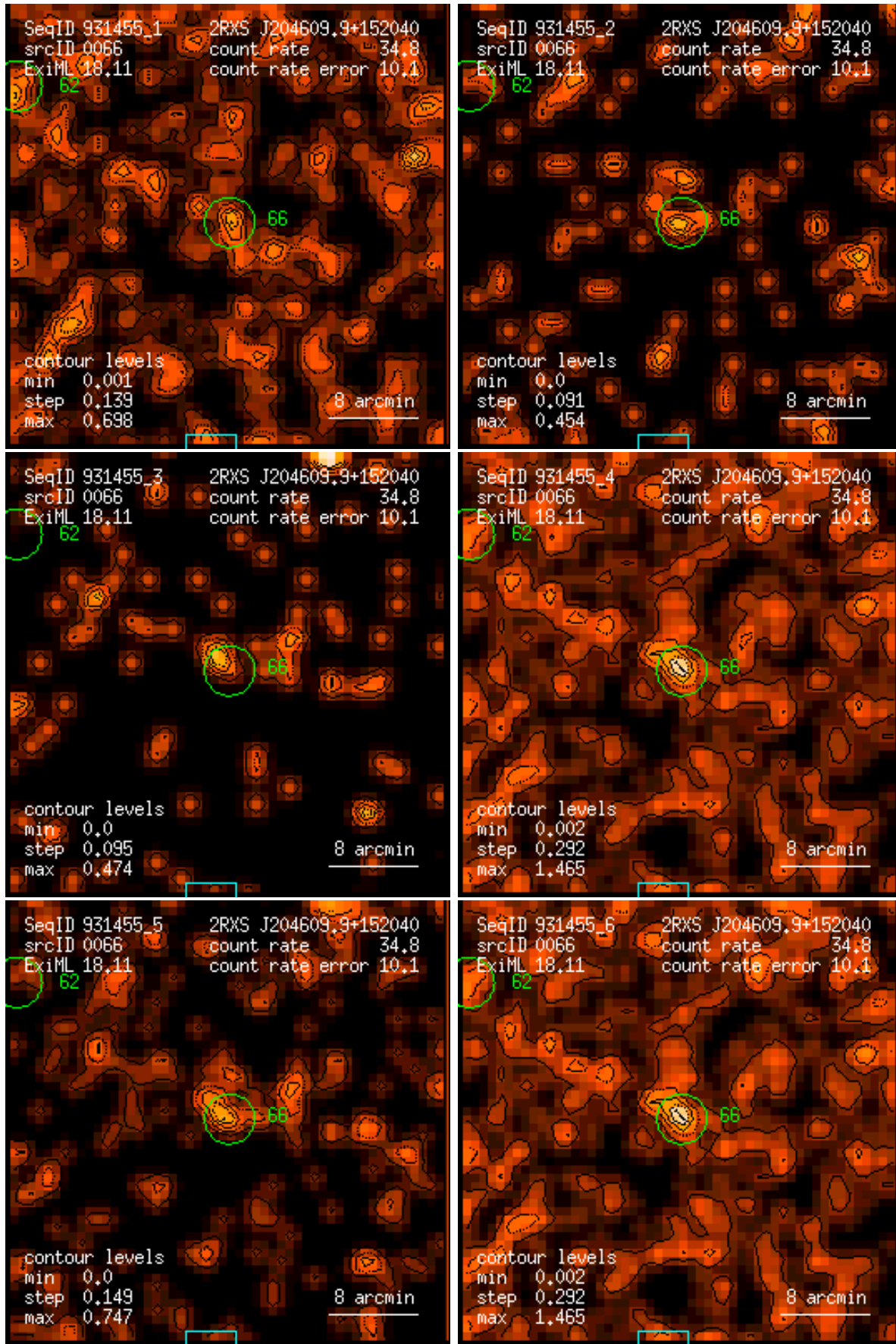
Figure 66: RASS 931455: detection 0066: band rate images, Gaussian filter: (1) PSPC channels 11 – 41, (2) 52 – 90, (3) 91 – 201, (4) 11 – 235, (5) 52 – 201, (6) 11 – 201. Broad band rates in counts/ks. Band rate contour levels in counts/ks/arcmin 2 .
