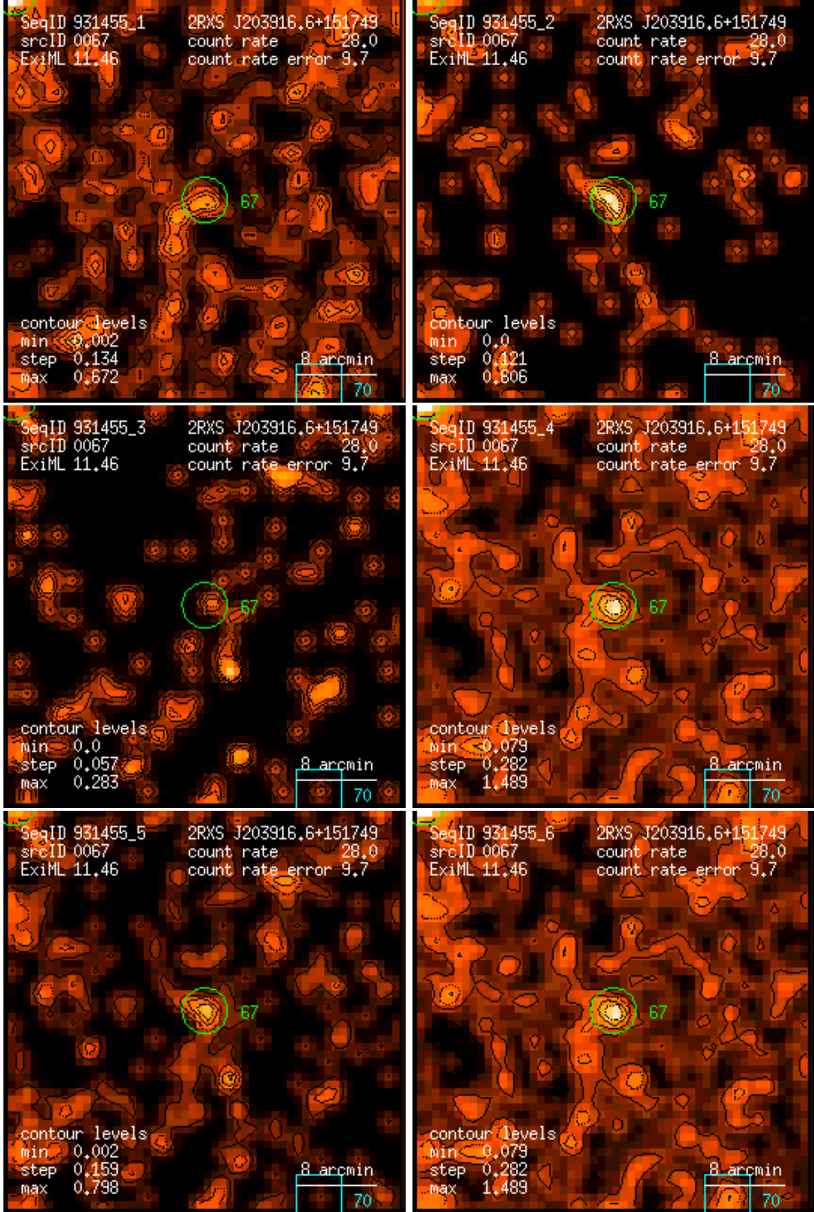
Figure 67: RASS 931455: detection 0067: band rate images, Gaussian filter: (1) PSPC channels 11 – 41, (2) 52 – 90, (3) 91 – 201, (4) 11 – 235, (5) 52 – 201, (6) 11 – 201. Broad band rates in counts/ks. Band rate contour levels in counts/ks/arcmin 2 .
