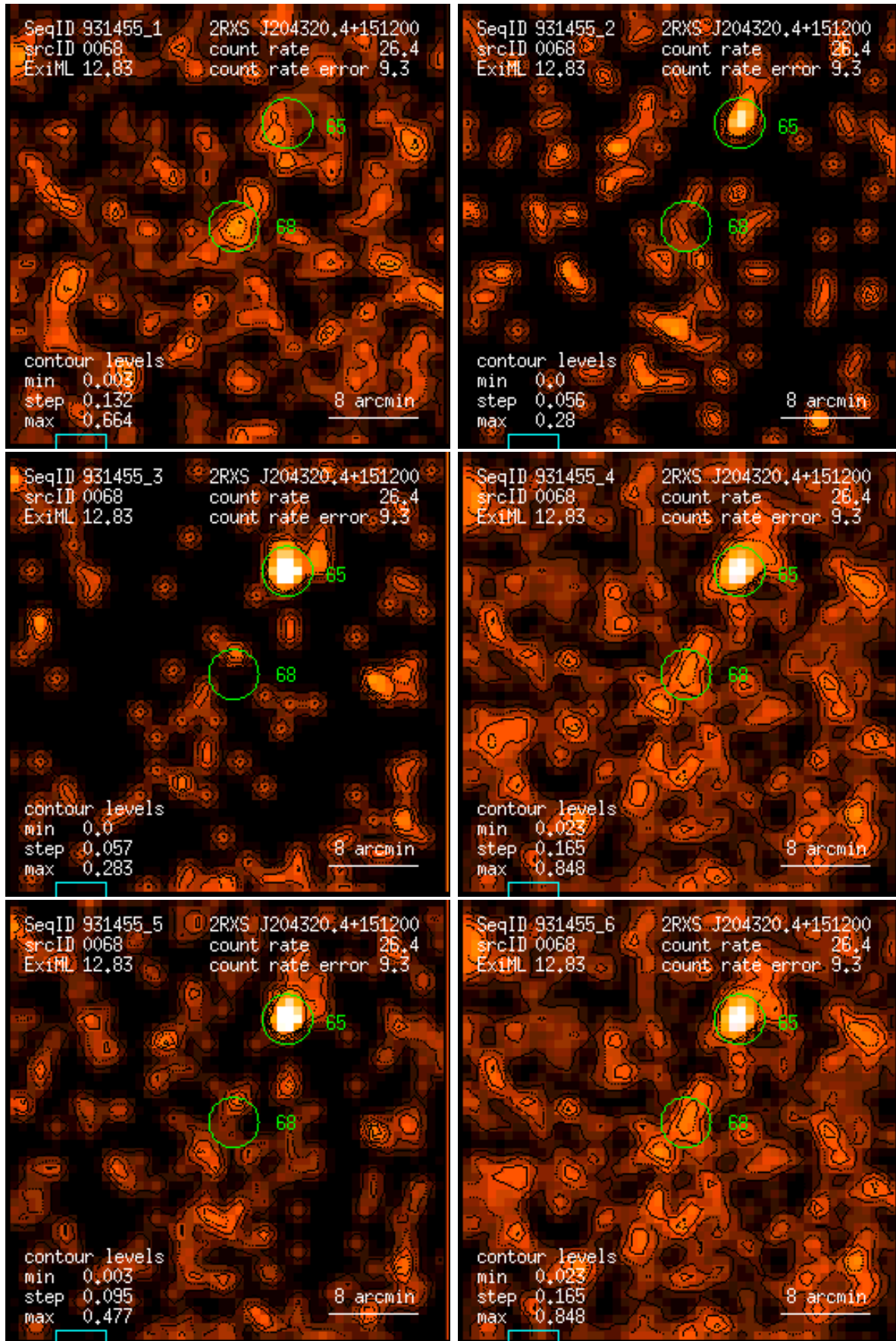
Figure 68: RASS 931455: detection 0068: band rate images, Gaussian filter: (1) PSPC channels 11 – 41, (2) 52 – 90, (3) 91 – 201, (4) 11 – 235, (5) 52 – 201, (6) 11 – 201. Broad band rates in counts/ks. Band rate contour levels in counts/ks/arcmin 2 .
