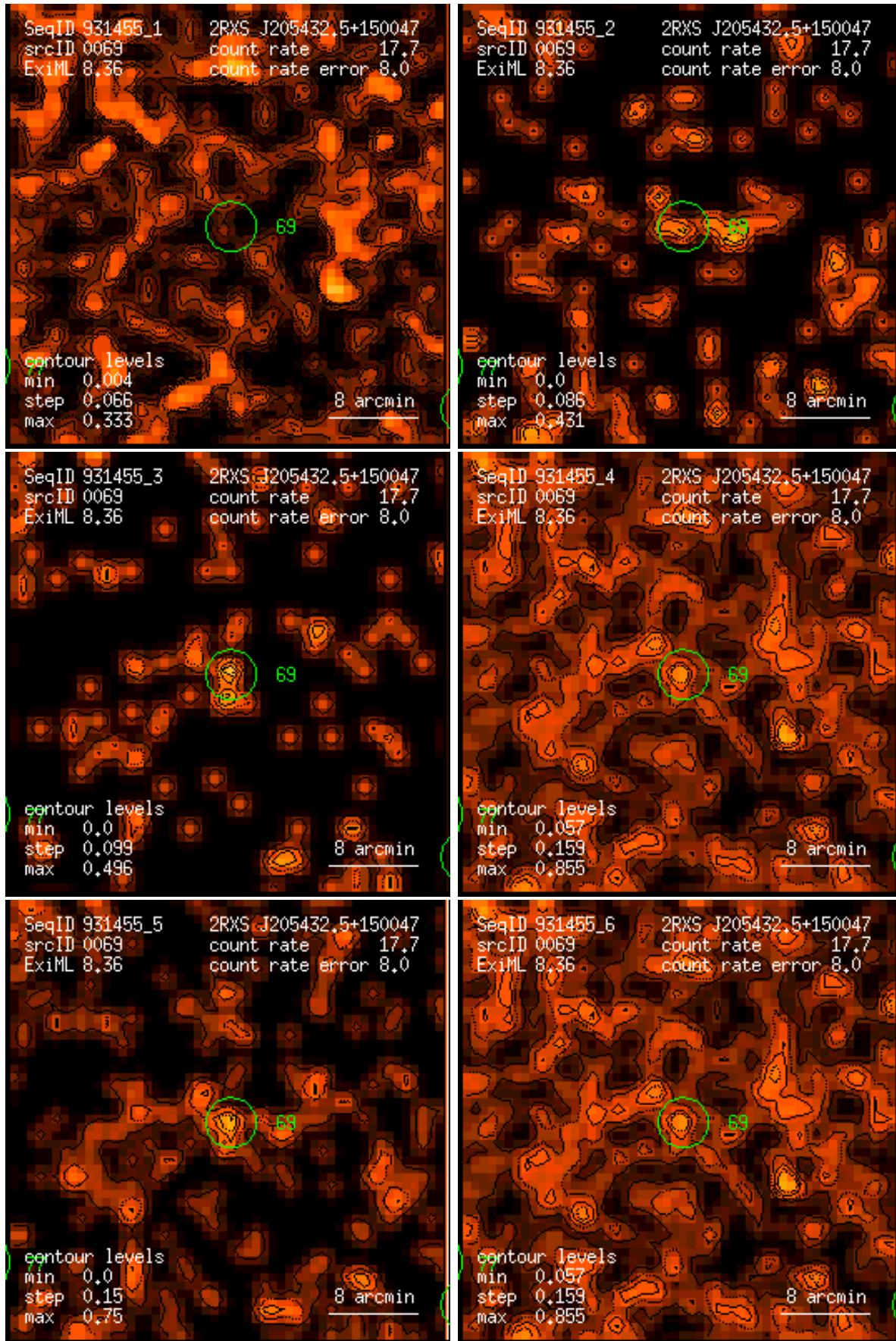
Figure 69: RASS 931455: detection 0069: band rate images, Gaussian filter: (1) PSPC channels 11 – 41, (2) 52 – 90, (3) 91 – 201, (4) 11 – 235, (5) 52 – 201, (6) 11 – 201. Broad band rates in counts/ks. Band rate contour levels in counts/ks/arcmin 2 .
