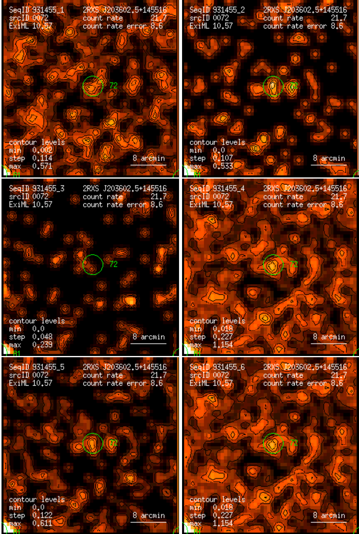
Figure 72: RASS 931455: detection 0072: band rate images, Gaussian filter: (1) PSPC channels 11 – 41, (2) 52 – 90, (3) 91 – 201, (4) 11 – 235, (5) 52 – 201, (6) 11 – 201. Broad band rates in counts/ks. Band rate contour levels in counts/ks/arcmin 2 .
