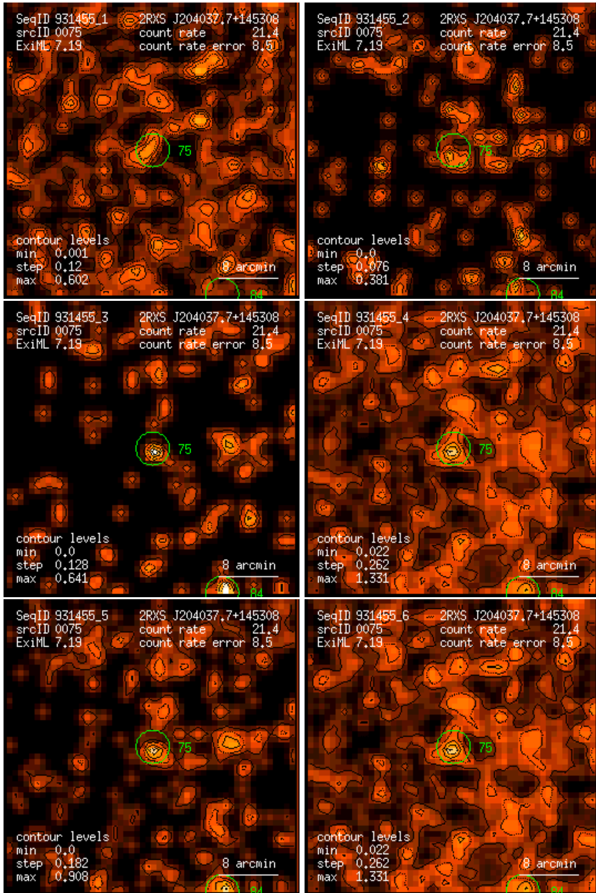
Figure 75: RASS 931455: detection 0075: band rate images, Gaussian filter: (1) PSPC channels 11 – 41, (2) 52 – 90, (3) 91 – 201, (4) 11 – 235, (5) 52 – 201, (6) 11 – 201. Broad band rates in counts/ks. Band rate contour levels in counts/ks/arcmin 2 .
