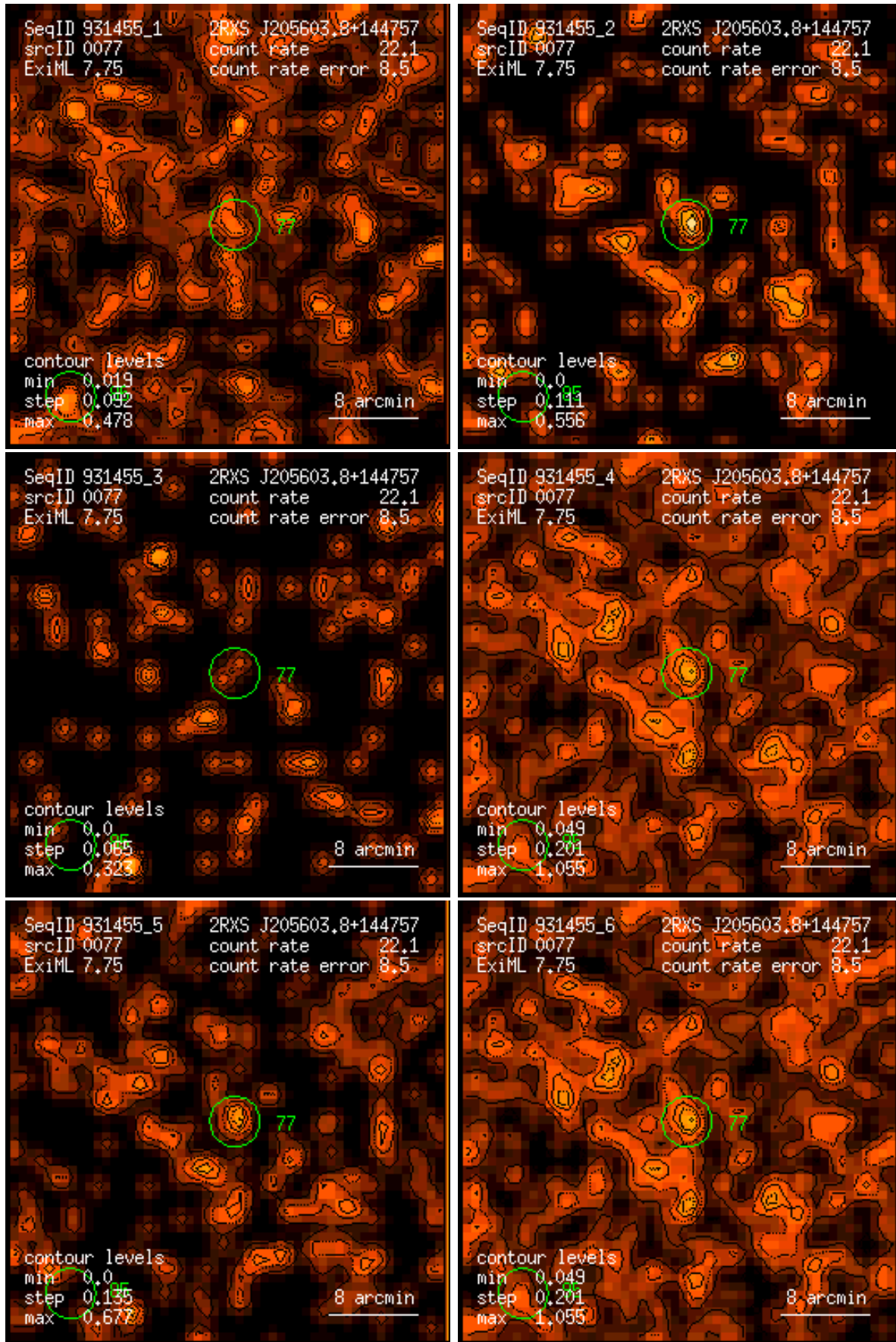
Figure 77: RASS 931455: detection 0077: band rate images, Gaussian filter: (1) PSPC channels 11 – 41, (2) 52 – 90, (3) 91 – 201, (4) 11 – 235, (5) 52 – 201, (6) 11 – 201. Broad band rates in counts/ks. Band rate contour levels in counts/ks/arcmin 2 .
