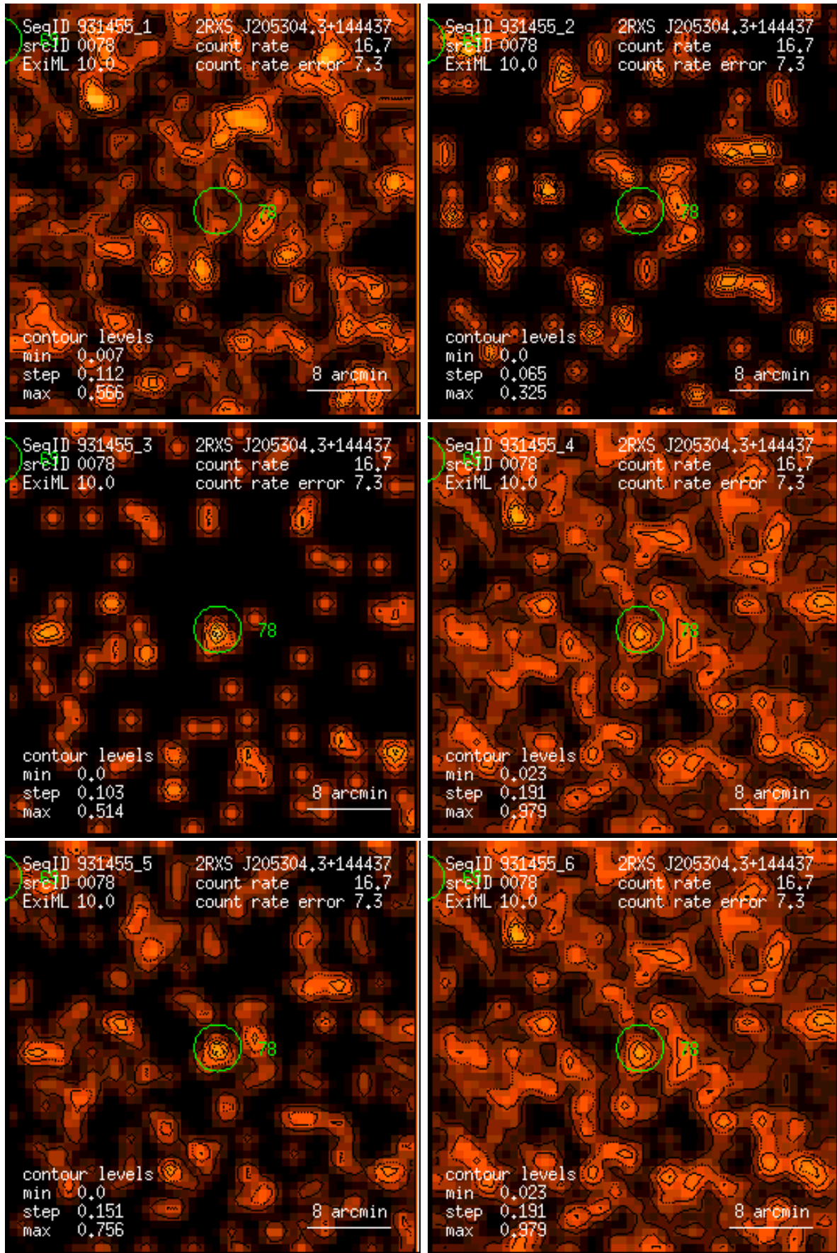
Figure 78: RASS 931455: detection 0078: band rate images, Gaussian filter: (1) PSPC channels 11 – 41, (2) 52 – 90, (3) 91 – 201, (4) 11 – 235, (5) 52 – 201, (6) 11 – 201. Broad band rates in counts/ks. Band rate contour levels in counts/ks/arcmin 2 .
