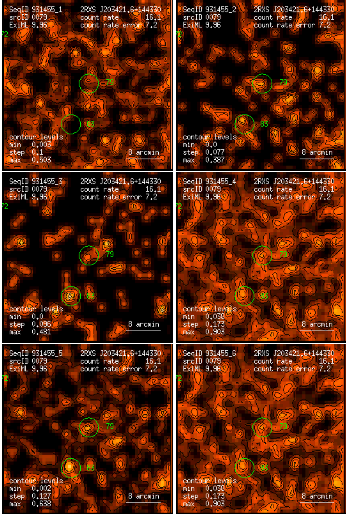
Figure 79: RASS 931455: detection 0079: band rate images, Gaussian filter: (1) PSPC channels 11 – 41, (2) 52 – 90, (3) 91 – 201, (4) 11 – 235, (5) 52 – 201, (6) 11 – 201. Broad band rates in counts/ks. Band rate contour levels in counts/ks/arcmin 2 .
