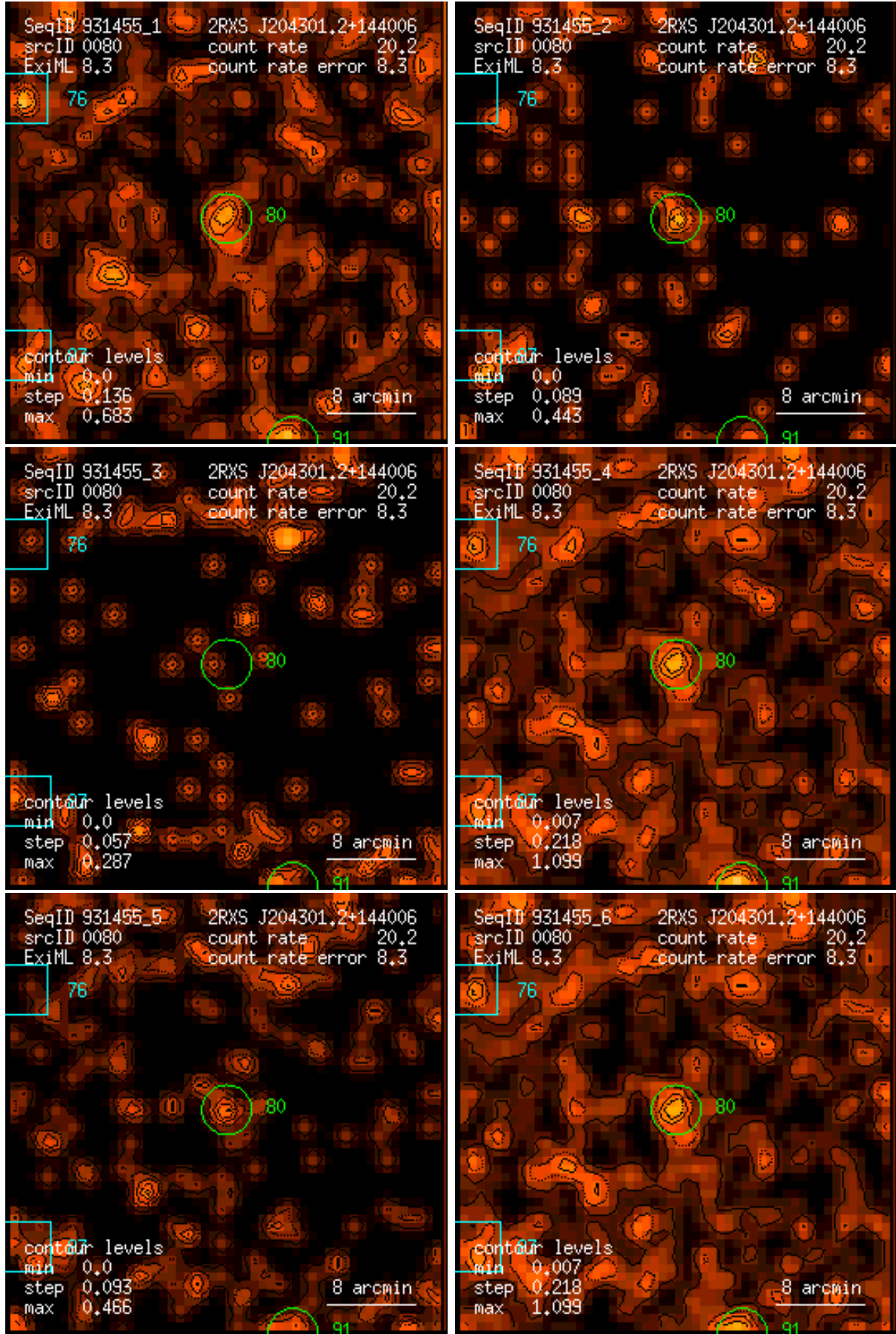
Figure 80: RASS 931455: detection 0080: band rate images, Gaussian filter: (1) PSPC channels 11 – 41, (2) 52 – 90, (3) 91 – 201, (4) 11 – 235, (5) 52 – 201, (6) 11 – 201. Broad band rates in counts/ks. Band rate contour levels in counts/ks/arcmin 2 .
