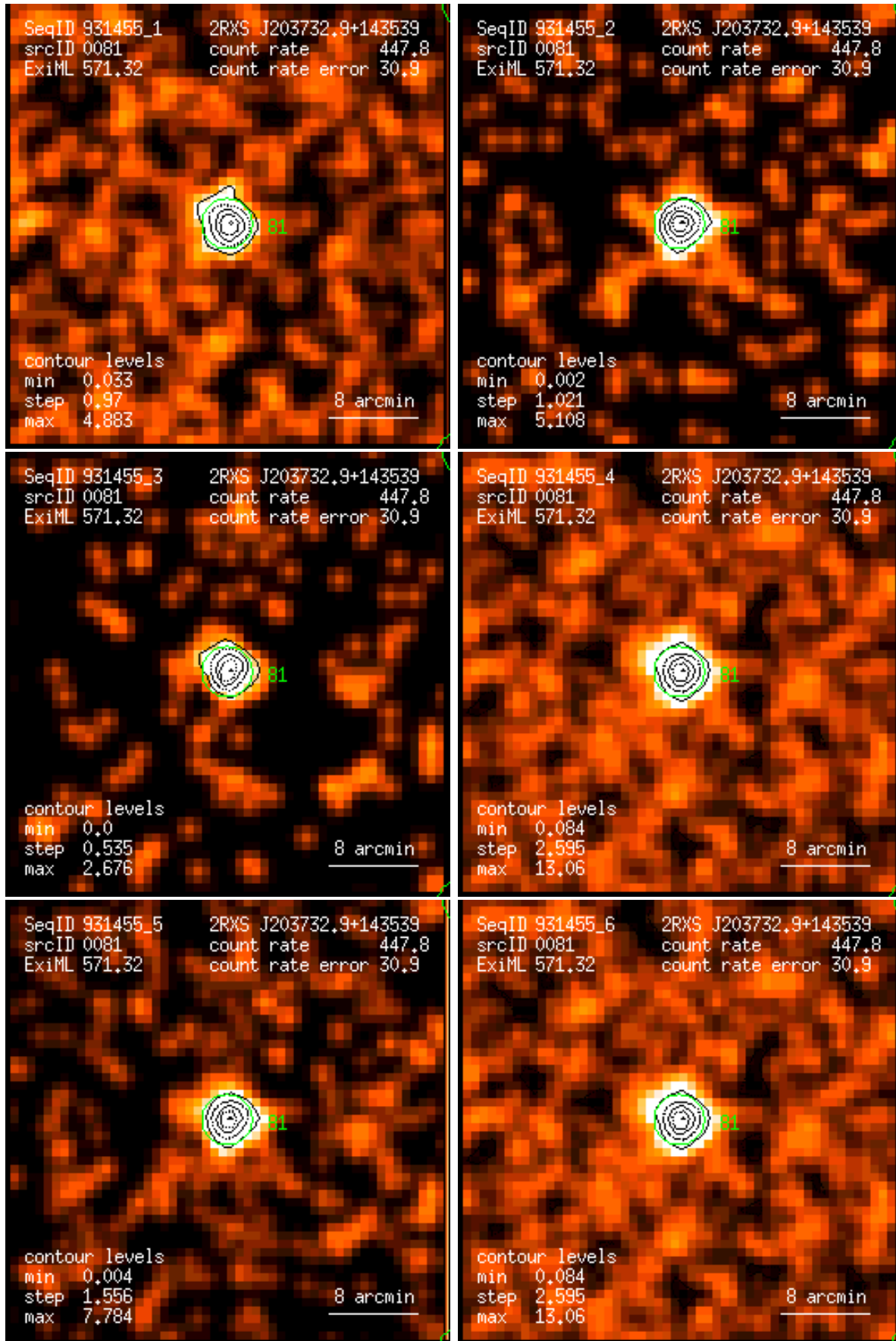
Figure 81: RASS 931455: detection 0081: band rate images, Gaussian filter: (1) PSPC channels 11 – 41, (2) 52 – 90, (3) 91 – 201, (4) 11 – 235, (5) 52 – 201, (6) 11 – 201. Broad band rates in counts/ks. Band rate contour levels in counts/ks/arcmin 2 .
