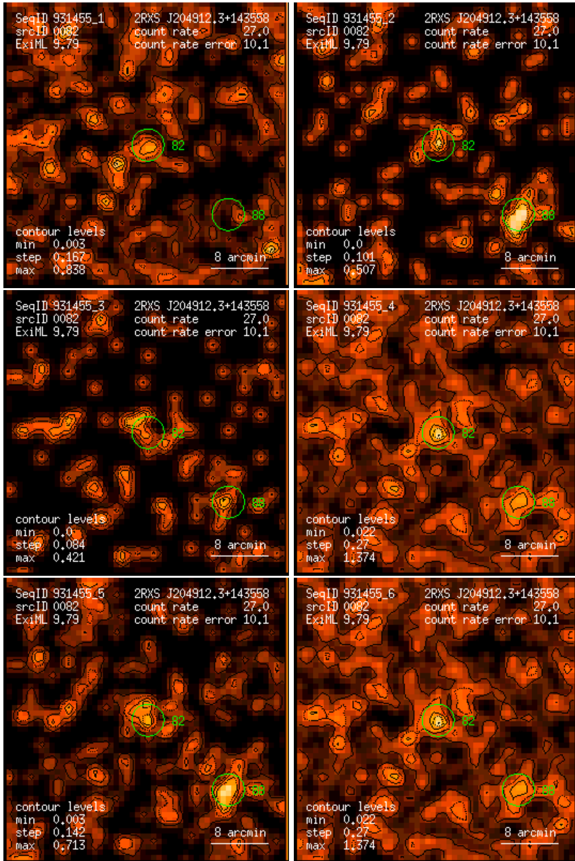
Figure 82: RASS 931455: detection 0082: band rate images, Gaussian filter: (1) PSPC channels 11 – 41, (2) 52 – 90, (3) 91 – 201, (4) 11 – 235, (5) 52 – 201, (6) 11 – 201. Broad band rates in counts/ks. Band rate contour levels in counts/ks/arcmin 2 .
