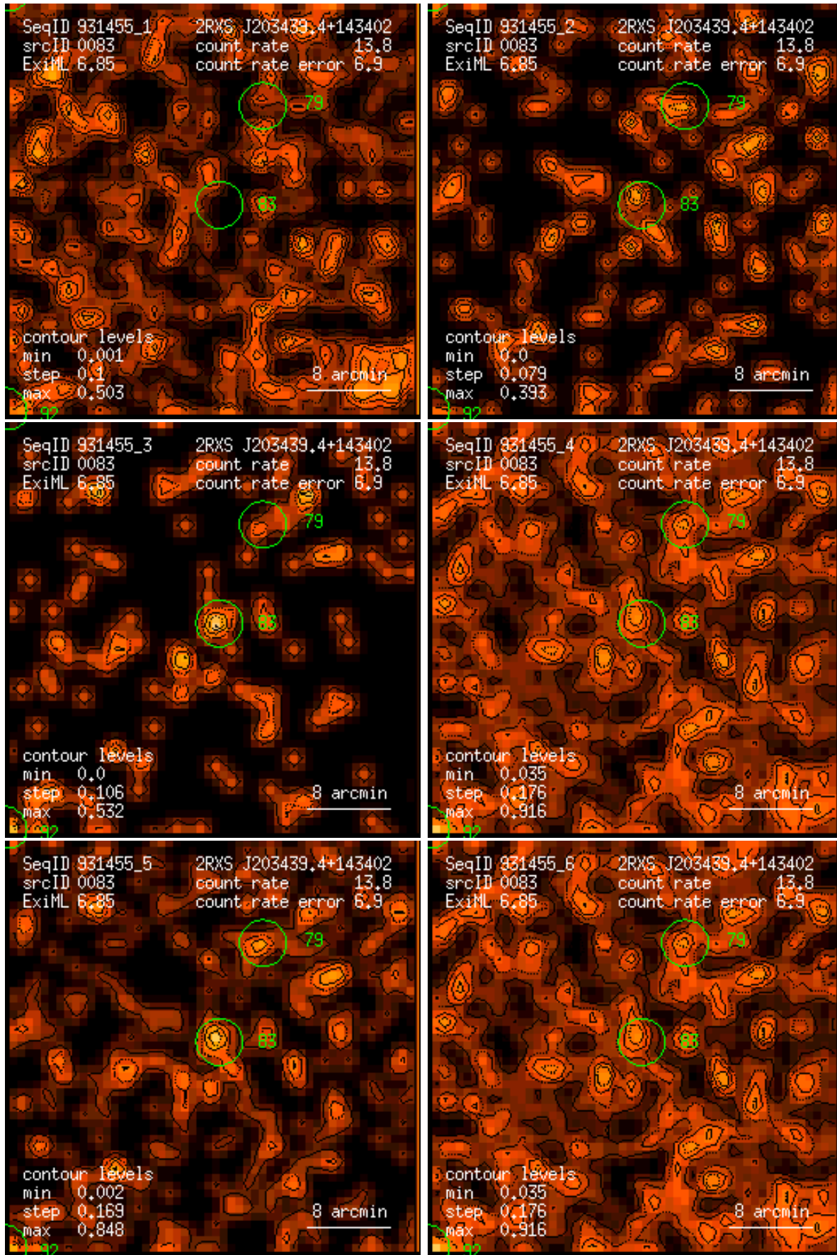
Figure 83: RASS 931455: detection 0083: band rate images, Gaussian filter: (1) PSPC channels 11 – 41, (2) 52 – 90, (3) 91 – 201, (4) 11 – 235, (5) 52 – 201, (6) 11 – 201. Broad band rates in counts/ks. Band rate contour levels in counts/ks/arcmin 2 .
