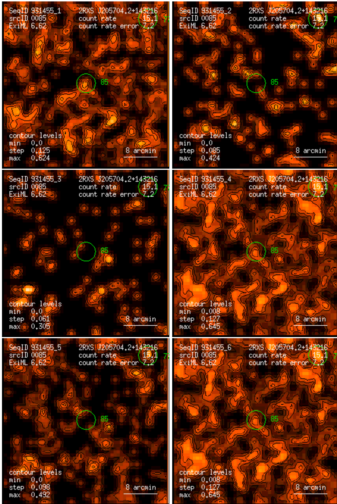
Figure 85: RASS 931455: detection 0085: band rate images, Gaussian filter: (1) PSPC channels 11 – 41, (2) 52 – 90, (3) 91 – 201, (4) 11 – 235, (5) 52 – 201, (6) 11 – 201. Broad band rates in counts/ks. Band rate contour levels in counts/ks/arcmin 2 .
