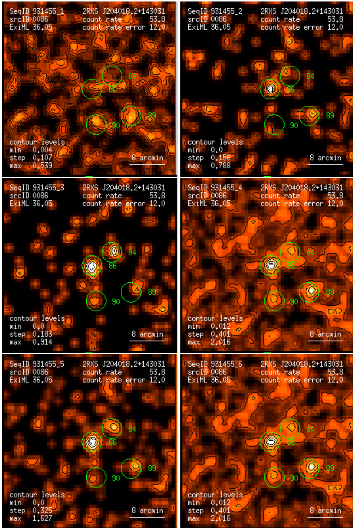
Figure 86: RASS 931455: detection 0086: band rate images, Gaussian filter: (1) PSPC channels 11 – 41, (2) 52 – 90, (3) 91 – 201, (4) 11 – 235, (5) 52 – 201, (6) 11 – 201. Broad band rates in counts/ks. Band rate contour levels in counts/ks/arcmin 2 .
