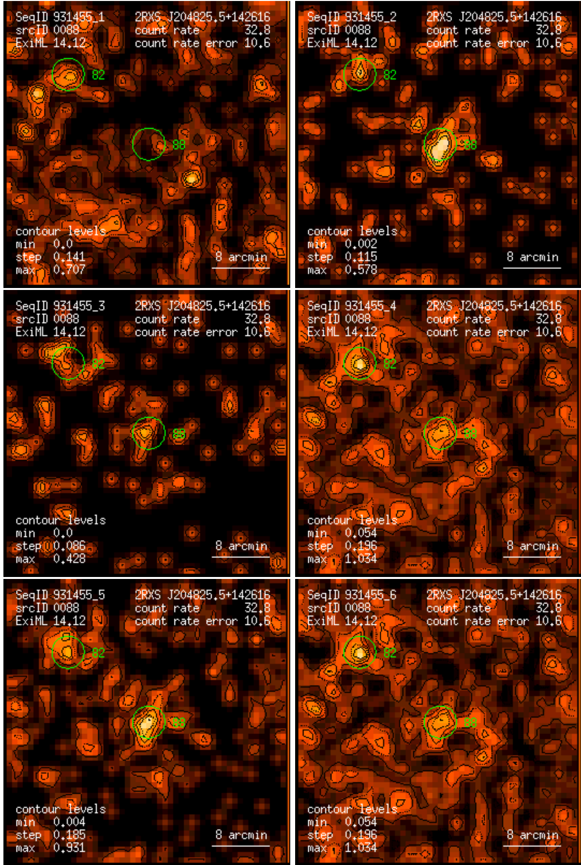
Figure 88: RASS 931455: detection 0088: band rate images, Gaussian filter: (1) PSPC channels 11 – 41, (2) 52 – 90, (3) 91 – 201, (4) 11 – 235, (5) 52 – 201, (6) 11 – 201. Broad band rates in counts/ks. Band rate contour levels in counts/ks/arcmin 2 .
