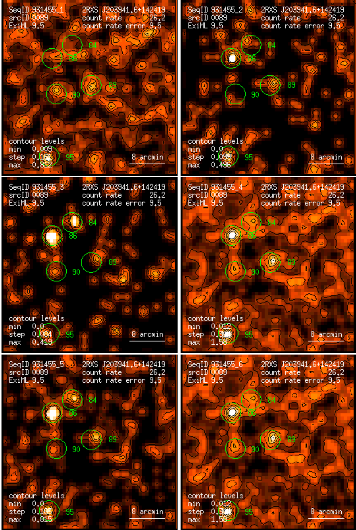
Figure 89: RASS 931455: detection 0089: band rate images, Gaussian filter: (1) PSPC channels 11 – 41, (2) 52 – 90, (3) 91 – 201, (4) 11 – 235, (5) 52 – 201, (6) 11 – 201. Broad band rates in counts/ks. Band rate contour levels in counts/ks/arcmin 2 .
