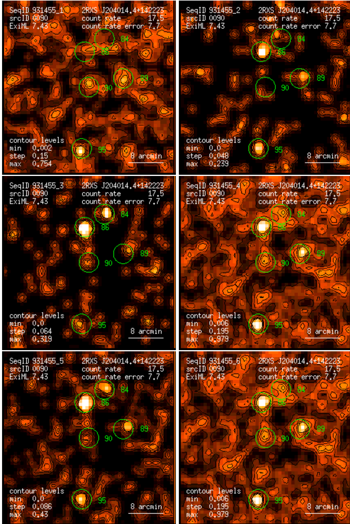
Figure 90: RASS 931455: detection 0090: band rate images, Gaussian filter: (1) PSPC channels 11 – 41, (2) 52 – 90, (3) 91 – 201, (4) 11 – 235, (5) 52 – 201, (6) 11 – 201. Broad band rates in counts/ks. Band rate contour levels in counts/ks/arcmin 2 .
