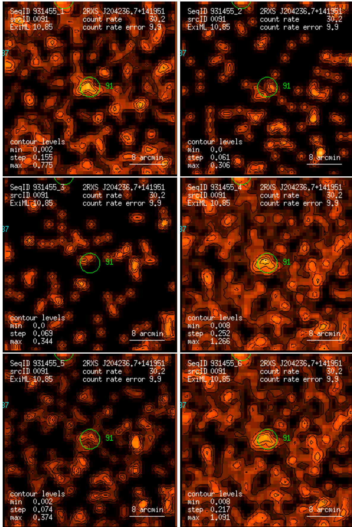
Figure 91: RASS 931455: detection 0091: band rate images, Gaussian filter: (1) PSPC channels 11 – 41, (2) 52 – 90, (3) 91 – 201, (4) 11 – 235, (5) 52 – 201, (6) 11 – 201. Broad band rates in counts/ks. Band rate contour levels in counts/ks/arcmin 2 .
