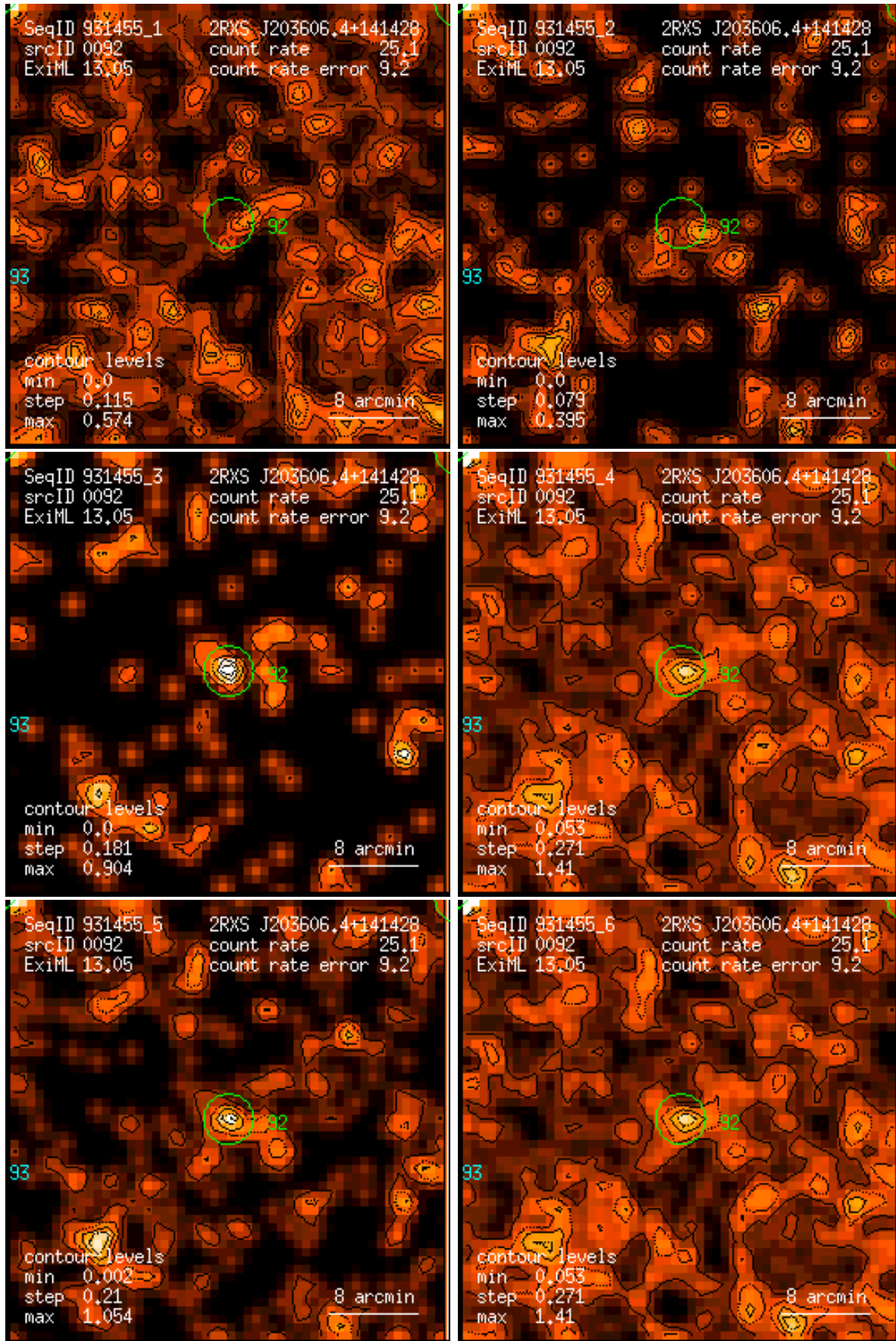
Figure 92: RASS 931455: detection 0092: band rate images, Gaussian filter: (1) PSPC channels 11 – 41, (2) 52 – 90, (3) 91 – 201, (4) 11 – 235, (5) 52 – 201, (6) 11 – 201. Broad band rates in counts/ks. Band rate contour levels in counts/ks/arcmin 2 .
