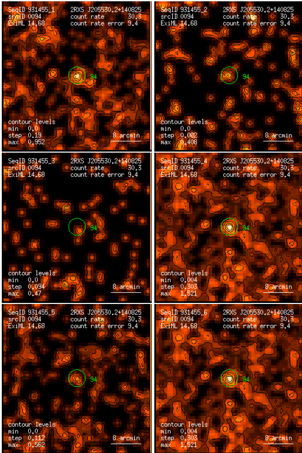
Figure 94: RASS 931455: detection 0094: band rate images, Gaussian filter: (1) PSPC channels 11 – 41, (2) 52 – 90, (3) 91 – 201, (4) 11 – 235, (5) 52 – 201, (6) 11 – 201. Broad band rates in counts/ks. Band rate contour levels in counts/ks/arcmin 2 .
