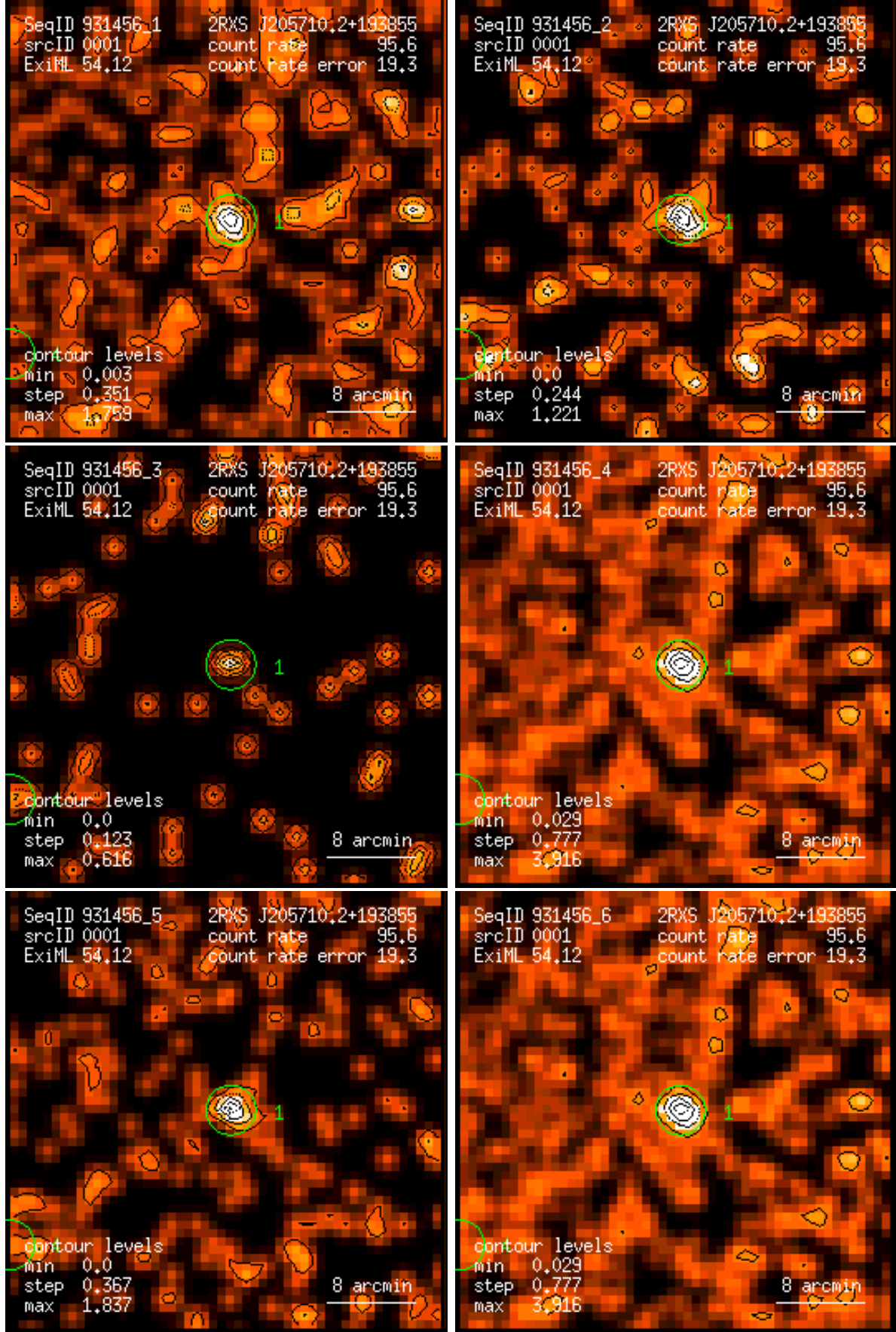
Figure 1: RASS 931456: detection 0001: band rate images, Gaussian filter: (1) PSPC channels 11 – 41, (2) 52 – 90, (3) 91 – 201, (4) 11 – 235, (5) 52 – 201, (6) 11 – 201. Broad band rates in counts/ks. Band rate contour levels in counts/ks/arcmin 2 .
