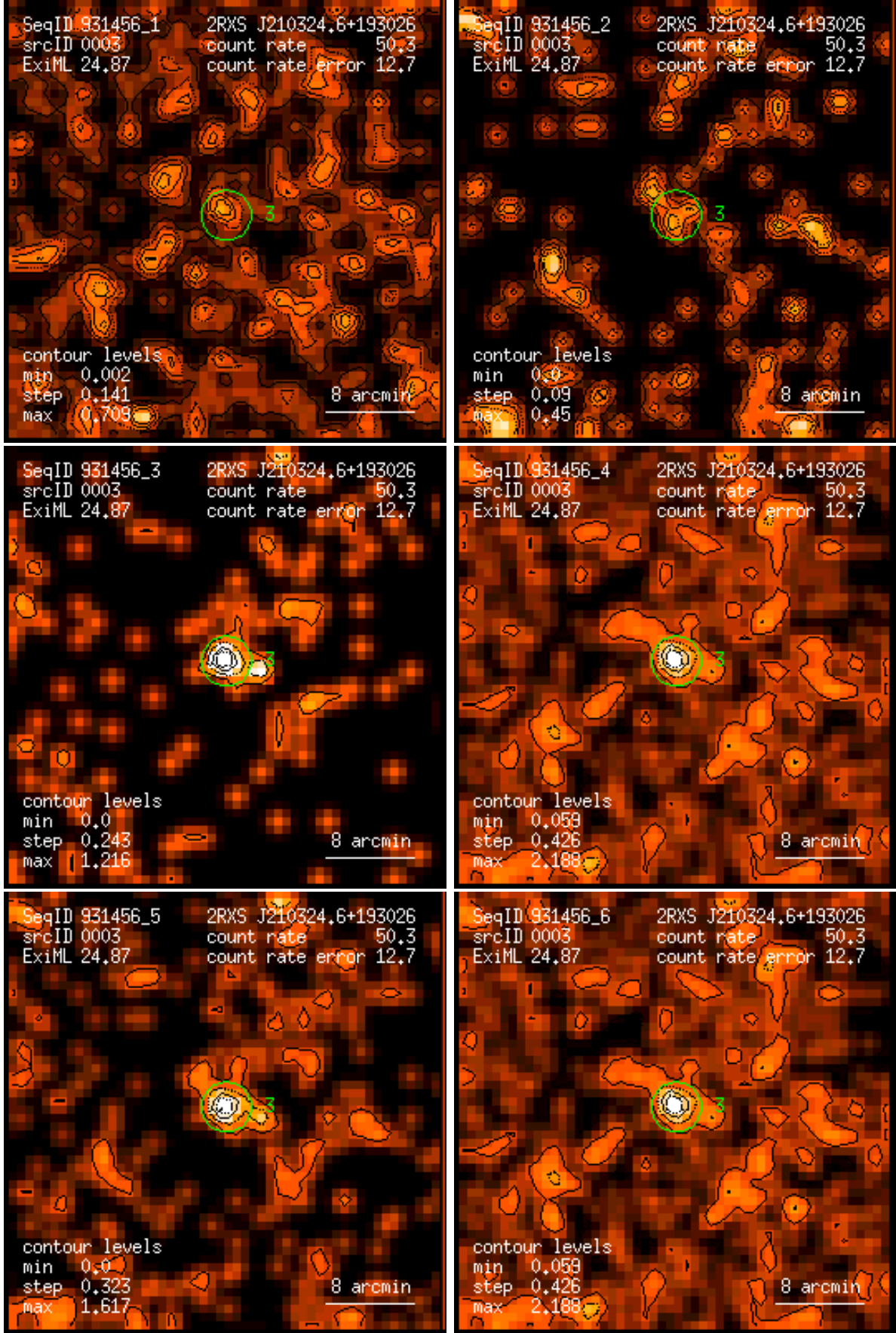
Figure 3: RASS 931456: detection 0003: band rate images, Gaussian filter: (1) PSPC channels 11 – 41, (2) 52 – 90, (3) 91 – 201, (4) 11 – 235, (5) 52 – 201, (6) 11 – 201. Broad band rates in counts/ks. Band rate contour levels in counts/ks/arcmin 2 .
